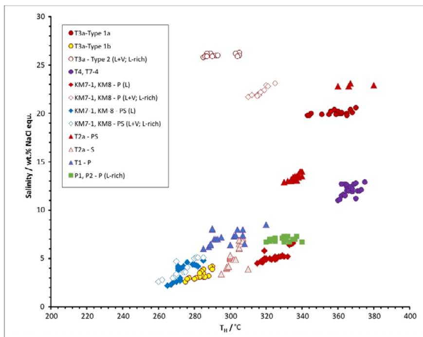
Figure 9. Correlation of homogenization temperature ( T_H ) and salinity for fluid inclusions hosted at contacts of the phreatomagmatic breccia and its host rocks as well as within different types of clasts and pyroclastic rocks.
