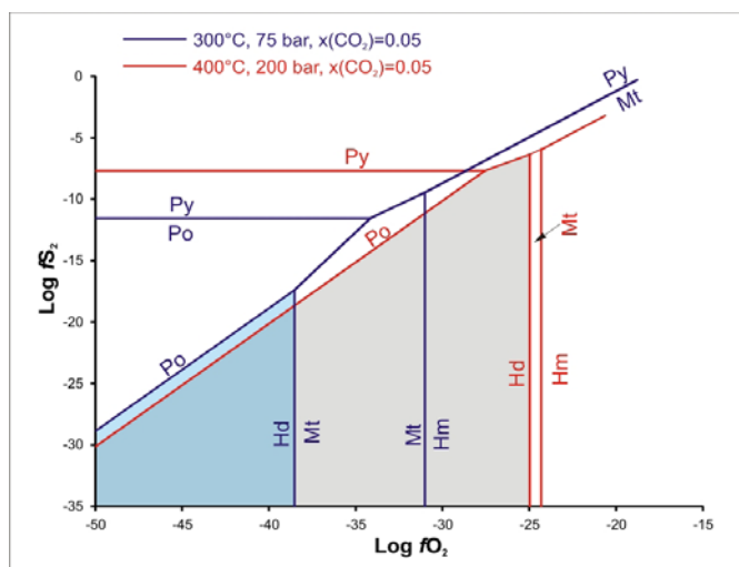
Figure 12. \text{Log } f_{\text{O}_2} vs. \text{log } f_{\text{S}_2} diagram of the Ca-Fe-Si-S-OH system constructed for the pre-breccia stage (lithostatic regime; P \approx 20 MPa; T \approx 400^\circ\text{C} ) and the main stage of the breccia formation (hydrostatic regime; P \approx 7.5 MPa; T \approx 300^\circ\text{C} ). The x(\text{CO}_2) value is set at 0.05.
