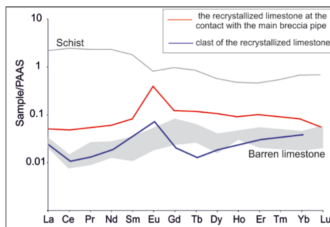
Figure 6. The post-Archean Australian shale (PAAS) normalized plots of the recrystallized limestone at the contact with the main breccia pipe and the recrystallized limestone clast from the main breccia pipe (75 m above mean sea level). The data for the schist and barren limestone are adopted from STRMIĆ PALINKAŠ et al. (2013).
