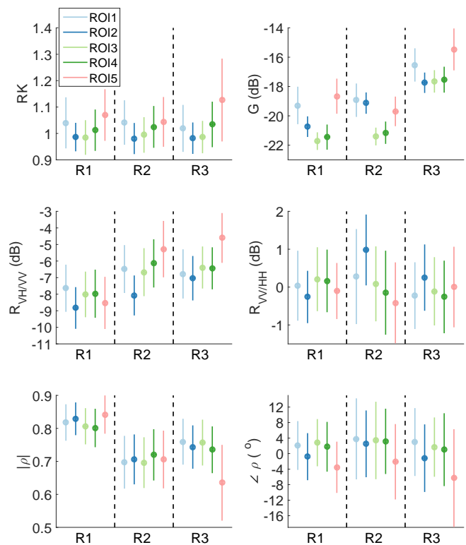
Figure 6. Mean values of the features in the regions of interest in the three RADARSAT-2 scenes (R1, R2 and R3). The error bars are 2 standard deviations long.
