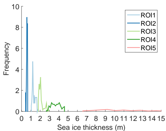
Figure 5. Histograms of sea ice thickness (m) measured during the helicopter flight 3 September 2011 for each of the five regions of interest (ROIs).
