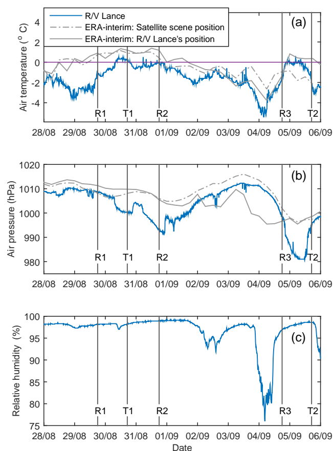
Figure 2. Air temperature (a), air pressure (b) and relative humidity (c) during the campaign. The grey vertical lines represent the time of the acquisition of the satellite scenes.
