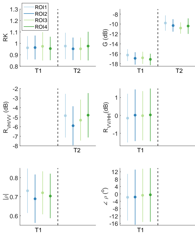
Figure 7. Mean values of the features in the regions of interest in the two TerraSAR-X scenes (T1 and T2). The error bars are 2 standard deviations long.
