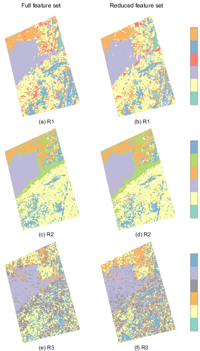
Figure 8. Segmentations of the three RADARSAT-2 scenes (R1, R2 and R3) into six segments. To the left: segmentation with full feature set. To the right: segmentation with reduced feature set consisting of relative kurtosis, geometric brightness, cross-polarisation ratio and co-polarisation angle.
