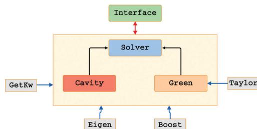
Fig. 1 Internal structure of the PCMSolver module.
