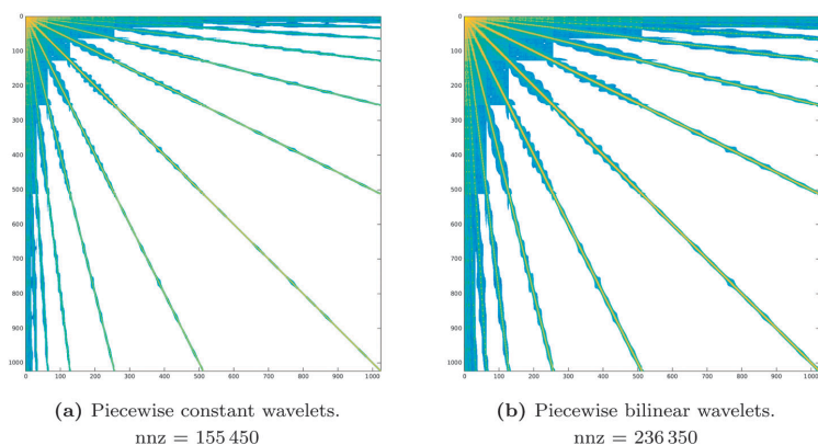
Fig. 8 Sparsity pattern for the system matrix representing the single layer operator \mathcal{S} as resulting from the first a priori compression only. The piecewise constant (left panel) and piecewise bilinear (right panel) wavelet bases are compared. In both cases the a priori compression parameters are kept fixed: a = 2.0 and d' = d'_{\max} .
