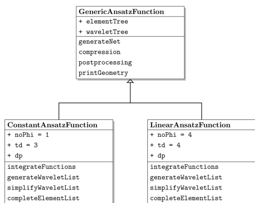
Fig. 4 Class diagram for the wavelet solver.
