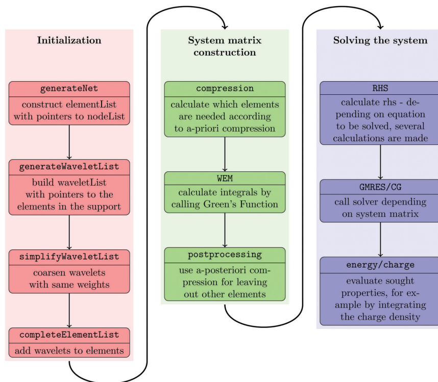
Fig. 2 Control flow for the wavelet solver.
