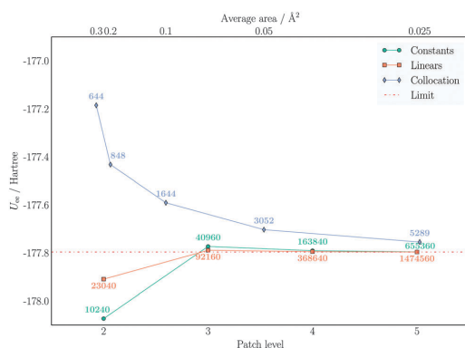
Fig. 10 Convergence of U_{\text{eo}} with respect to the number of molecular electrostatic potential (MEP) evaluation points on the cavity surface. The values reported are in Hartree and refer to benzene. The Gaussian basis 6-31G was used. The upper axis reports the average area for the collocation tessellation, while the lower axis refers to the patch level in the wavelet Galerkin discretization. The annotation report the number of MEP evaluation points. The compression parameter triplet was set to a = 2.5 , d' = 2.0 , b = 0.01 for the piecewise constant wavelets and to a = 2.5 , d' = 3.0 , b = 0.01 for piecewise bilinear wavelets. The limit value is extrapolated from the results obtained from the piecewise bilinear wavelet Galerkin scheme.
