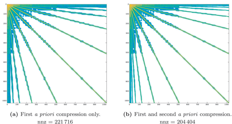
Fig. 7 Sparsity pattern for the system matrix representing the single layer operator \mathcal{S} in a piecewise bilinear wavelet basis. The effect of the first a priori compression (left panel) is compared to the combined effect of the first and second a priori compression (right panel). Both parameters are kept fixed: a = 2.0 and d' = d'_{1/2} . The number of non-zero elements (nnz) is reported under each matrix.
