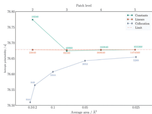
Fig. 12 Convergence of \alpha_{\text{iso}} with respect to the number of molecular electrostatic potential (MEP) evaluation points on the cavity surface. The values reported are in \text{Å}^3 and refer to benzene. The lower axis reports the average area for the collocation tessellation, while the upper axis refers to the patch level in the wavelet Galerkin discretization. The annotation report the number of MEP evaluation points. The compression parameter triplet was set to a = 2.5 , d' = 2.0 , b = 0.01 for the piecewise constant wavelets and to a = 2.5 , d' = 3.0 , b = 0.01 for piecewise bilinear wavelets. The limit value is extrapolated from the results obtained from the piecewise bilinear wavelet Galerkin scheme.
