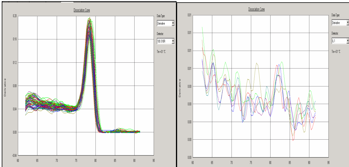
Figure 5: Disassociation/melting point (Tm) plot. The rate of change of the relative fluorescence units (RFU) with time (T) (-d(RFU)/dT) on the Y-axis versus the temperature on the X-axis. Left: Tm curve for 18S. The strands are showing similar melting points. Right: Faulty detection of primer-dimer artefacts are possible using sybr green, and this will give lower and fluctuated melting points due to shorter DNA strands, as shown here. Compared to the collective peak to the right.
