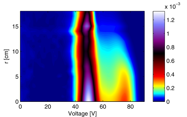
FIG. 15. RFEA measurements in Njord at 1.5 sccm.
