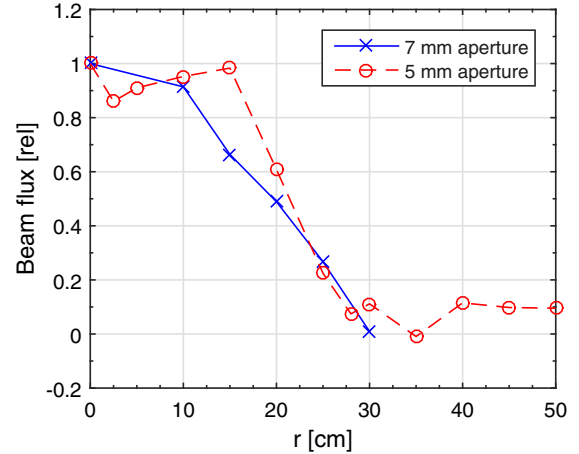
FIG. 10. Measured beam flux from the RFEA probe normalized to the beam flux in the center. Two different probe configurations were used. One with a 7 mm aperture and one with a 5 mm aperture.
