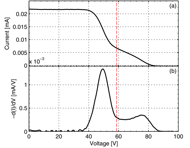
FIG. 4. RFEA-measurements in Njord at P = 0.28 mTorr with a magnetic field of 200 G in the source and 29 G in the expansion chamber. RF power is 1000 W. The measurement is taken at z = 55 cm, 11 cm from the end of the source and radially centered (Figure 2). The red dashed line marks the separation between beam and background distribution found by the algorithm.
