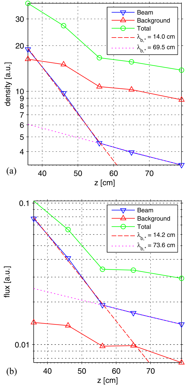
FIG. 8. Integrated beam and background densities (a) and flux (b) calculated from the LIF measurements in Figure 7(a).
