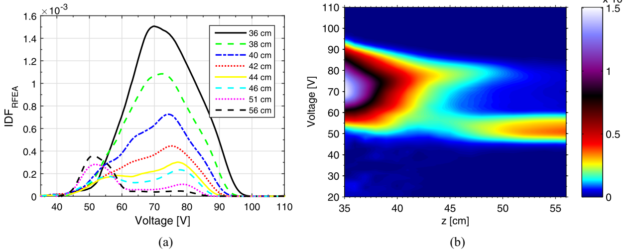
FIG. 13. RFEA measurements along the central z -axis of Njord. (a) IDFs at eight different positions. (b) A contour plot of IDFs for every cm from z = 36 to z = 56 cm. The colors represent the signal on the y -axis on (a). Discriminator voltage is displayed along the vertical axis. Both are obtained with a flow of 1.5 sccm resulting in a pressure of 2.8 \times 10^{-4} Torr in the expansion chamber.
