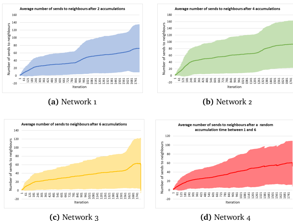
Figure 8.4: Figures show average number of sends from nodes (dark colors) to neighbour nodes for 100 nodes per network with different accumulation intervals with standard deviation (lighter colors).
