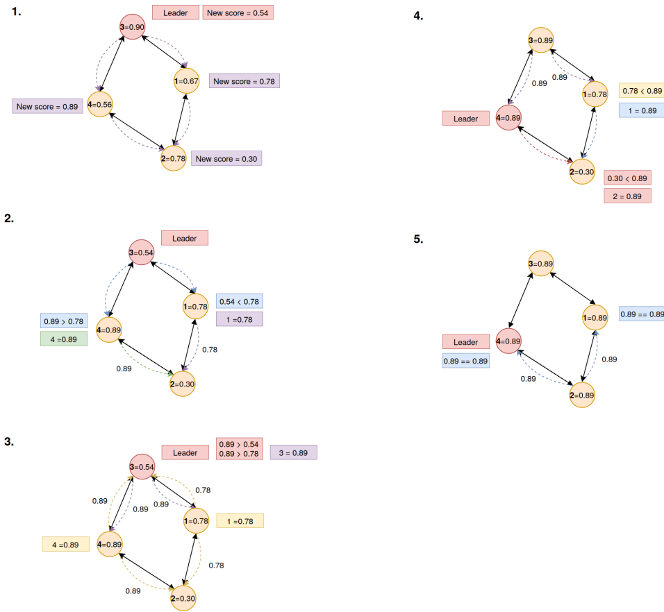
Figure 6.4: Figure show how a CH starts a CH-election.
