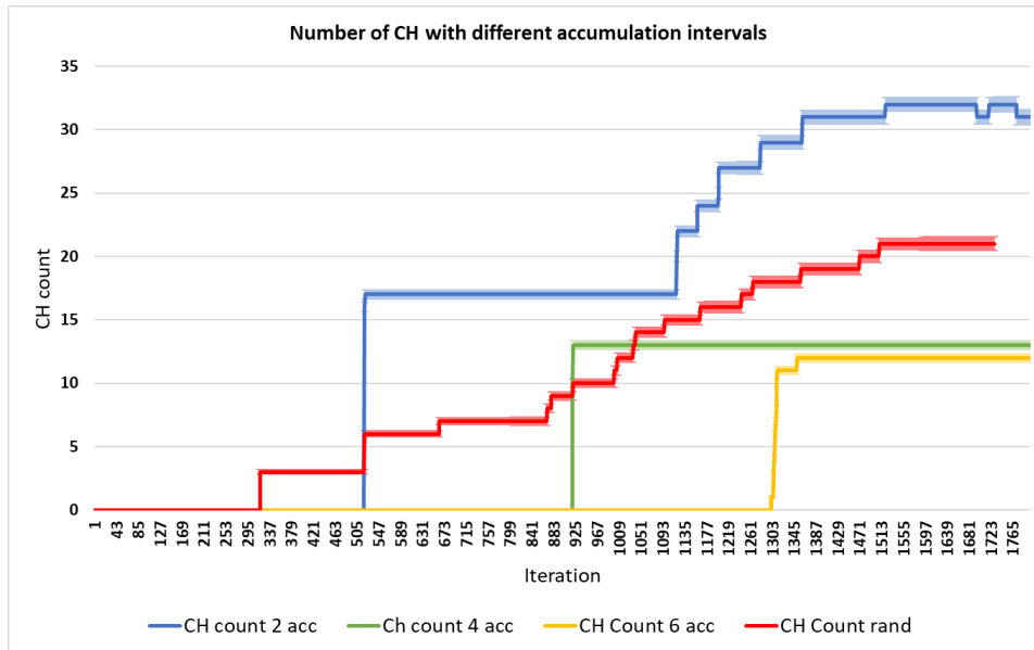
Figure 8.6: Figure shows the number of CHs for 100 nodes per network with different accumulation intervals.
