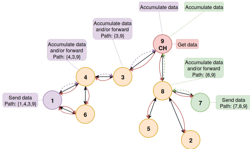
Figure 6.5: Figure show how a CH gossips a GET-data request and how nodes sends their data to the CH through the nodes in the path.
