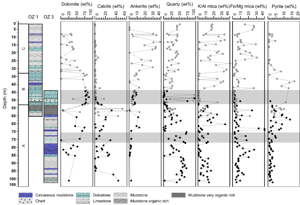
Figure 4. Generalised lithostratigraphic profile of the OnZap section divided into Units A to C (see text for details) and XRD-derived distributions of select mineral phases. The two OnZap cores are correlated using the base of a dolomite-chert unit occurring at 53 m in OnZap1 and at 10.8 m in OnZap3. Horizontal grey-shaded bars show intervals with evidence for secondary alteration. Grey and black data points denote samples from OnZap 1 and OnZap 3, respectively.
