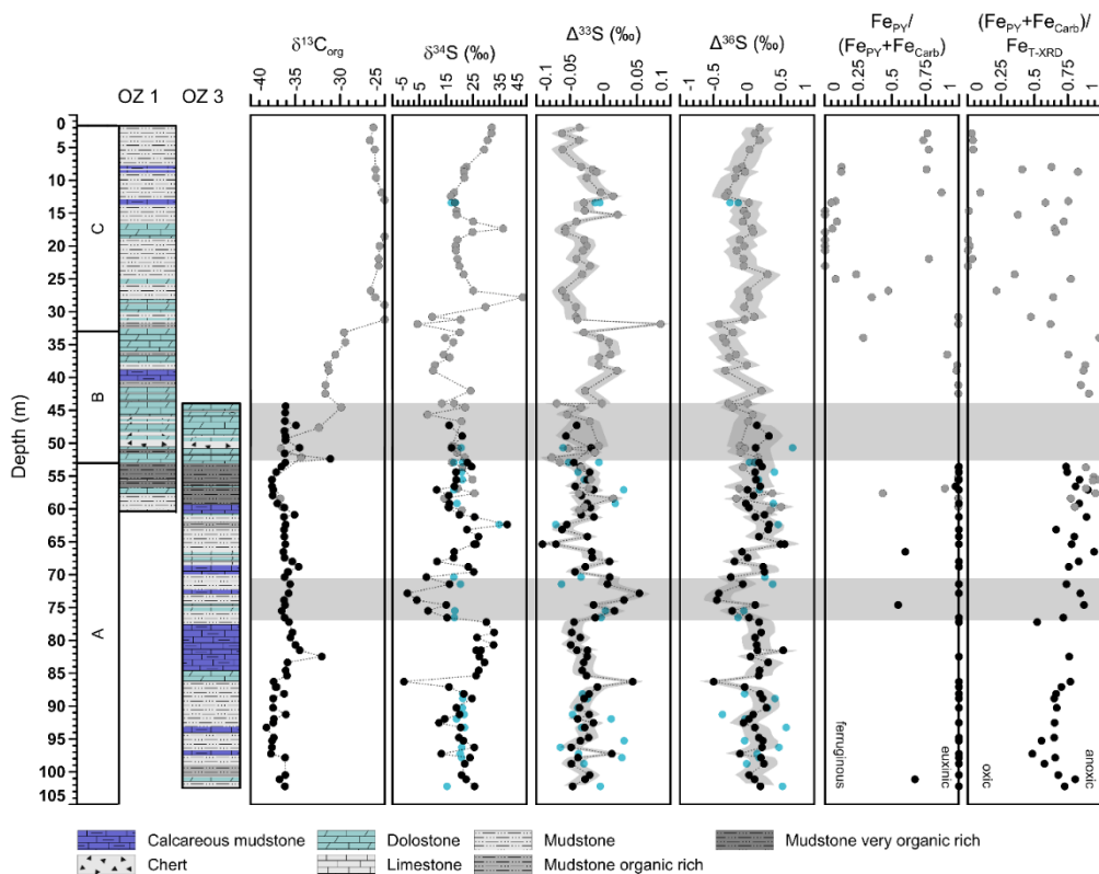
Figure 6. Generalised lithostratigraphic profile of the OnZap section divided into Units A to C (see text for details) plotted alongside carbon and sulphur isotope data and XRD-derived iron distribution data. The two OnZap cores are correlated using the base of a dolomite-chert unit occurring at 53 m in OnZap1 and at 10.8 m in OnZap3. Horizontal grey-shaded areas show intervals with evidence for secondary alteration. Grey and black data points denote samples from OnZap 1 and OnZap 3, respectively, whereas blue dots represent AVS results. Errors for the \delta^{13}\text{C}_{\text{org}} and \delta^{34}\text{S} are encompassed within the data points whereas the grey-shaded envelope illustrates the 1\sigma estimates of the analytical uncertainty for the \Delta^{33}\text{S} (0.015‰) and \Delta^{36}\text{S} (0.2‰) data.
