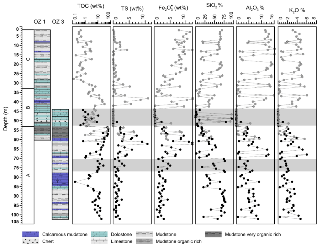
Figure 5. Generalised lithostratigraphic profile of the OnZap section divided into Units A to C (see text for details) plotted alongside selected components (TOC; TS; Fe 2 O 3 ; SiO 2 ; Al 2 O 3 and K 2 O). The two OnZap cores are correlated using the base of a dolomite-chert unit occurring at 53 m in OnZap1 and at 10.8 m in OnZap3. Horizontal grey-shaded bars show intervals with evidence for secondary alteration. Grey and black data points denote samples from OnZap1 and OnZap3, respectively.
