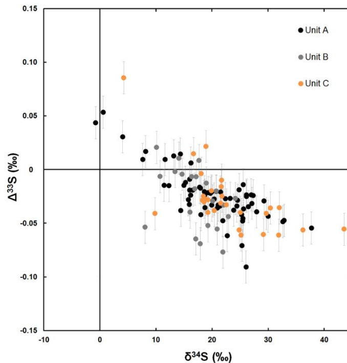
Figure 8. Triple-isotope plot of the pyrite sulphur isotope data for the entire OnZap section. Black circles are derived from Unit A, grey circles from Unit B and orange circles from Unit C. Uncertainties in the \Delta^{33}\text{S} values (0.015‰) are illustrated in grey, whereas the uncertainty in \delta^{34}\text{S} values are encompassed within each data point.
