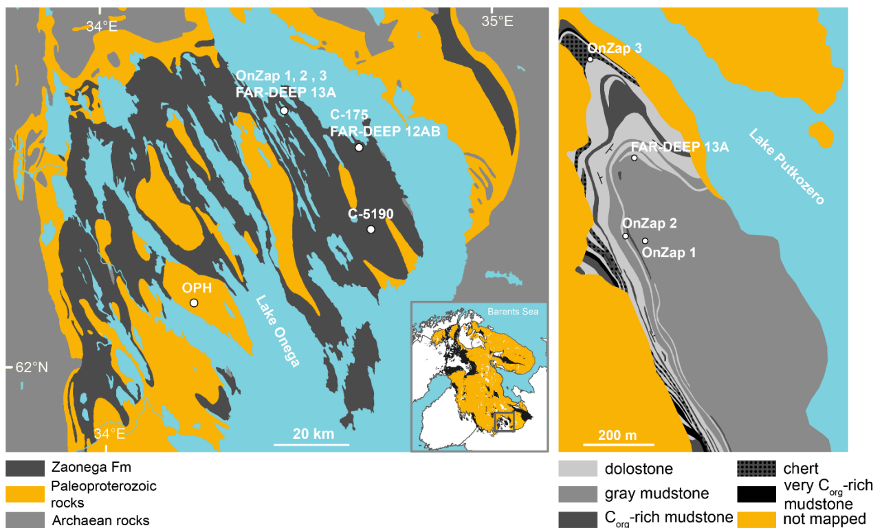
Figure 1. A. Simplified geological map of the Onega basin, NW Russia. Circles show locations of the OnZap 1 and 3 holes, FAR-DEEP holes 12AB, 13A, Onega Parametric Hole (OPH) and the C-175 and C-5190 holes. Inset map shows location of the Onega basin and occurrence of Paleoproterozoic rocks (black) across the eastern Fennoscandian Shield. B. Simplified geological map of the Zaonega Formation (after Melezhik et al., 2013a) near locations of OnZap 1 and 3 holes and FAR-DEEP hole 13A.
