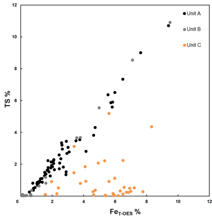
Figure 7. Sulphur (TS) and iron (Fe T-OES ) concentrations for the entire OnZap section. Black circles are derived from Unit A, grey circles from Unit B and orange circles from Unit C. Errors are encompassed within each data point.
