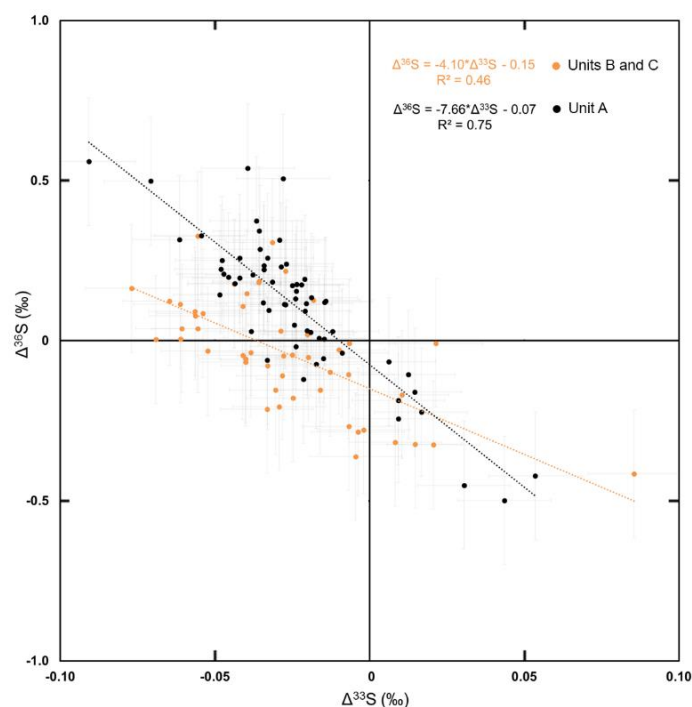
Figure 9. Quadruple-isotope plot of the pyrite sulphur isotope data for the entire OnZap section. Black circles are derived from Unit A and orange circles are from Units B and C. The dashed lines are regressions through the datasets derived from Unit A (-7.66; black) and Units B and C (-4.10; orange). The analytical uncertainties ( 1\sigma ) in both \Delta^{33}\text{S} (0.015‰) and \Delta^{36}\text{S} (0.2‰) are illustrated in grey.
