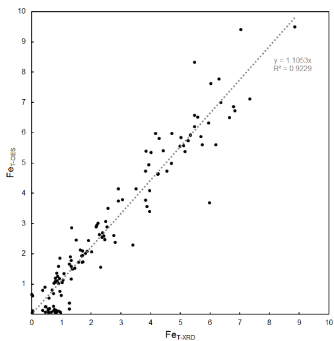
Supplementary figure 1. Comparison of the calculated Fe T-XRD and total Fe determined by ICP-OES (Fe T-OES ). The Fe T-OES and Fe T-XRD converge on a trend line with a slope of 1.1053 and R^2 = 0.92 .
