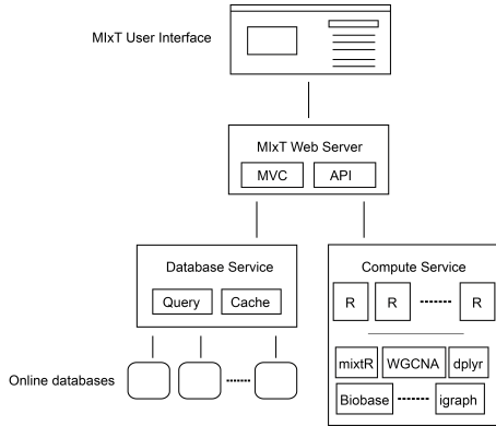
Figure 1: The architecture of the MIXT system. It consists of a web application, the hosting web server, a database service for retrieving metadata and a compute service for performing statistical analysis. Note that only the web application and the R package are specific to MIXT, the rest of the components can be reused in other applications.
