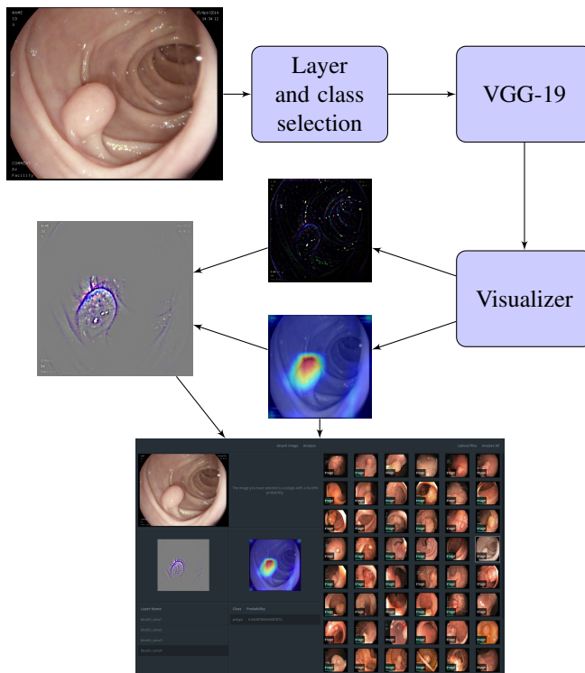
Fig. 1: An overview of how we produce the two visualisations included in the image analysis, and how it is presented in the user interface where a visualisation of the different convolutional layers can be selected.
