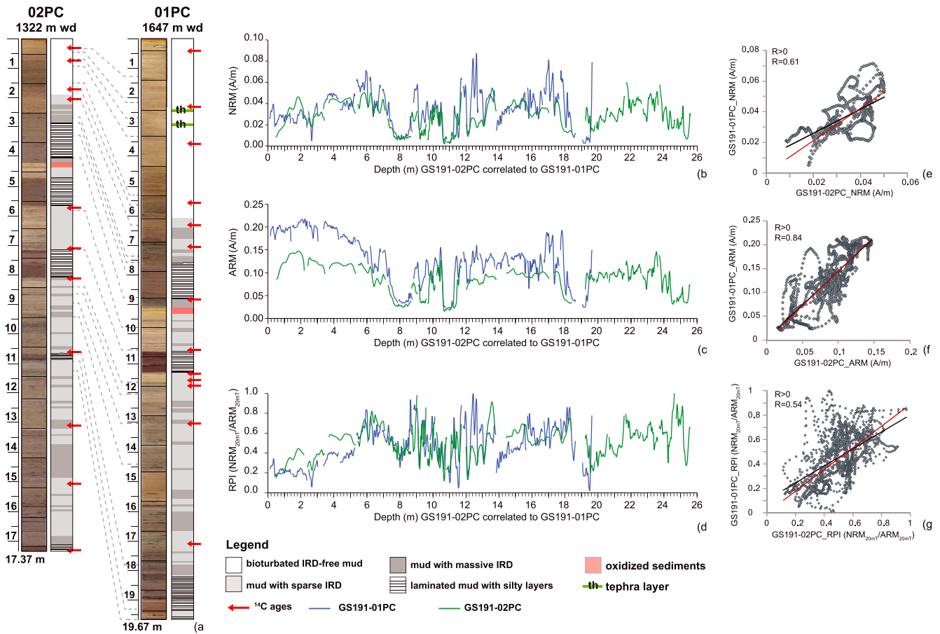
Figure 8. (a) Cores correlation stratigraphy, the red arrows indicate the ^{14}\text{C} ages, and the gray dashed line indicate correlation between the adopted tie points; (b) natural remanent magnetization (NRM); (c) anhysteretic remanent magnetization (ARM); and (d) relative paleointensity (RPI) curves. In the correlation procedure (Sagnotti & Caricchi, 2018), all data of core GS191-02PC (green) have been transferred to the stratigraphic depth of GS191-01PC (blue). Following the correlation procedure, the (e) NRM, (b) ARM, and (c) RPI curves of the two cores match with a correlation coefficient R = 0.61 , R = 0.84 , and R = 0.54 , respectively.
