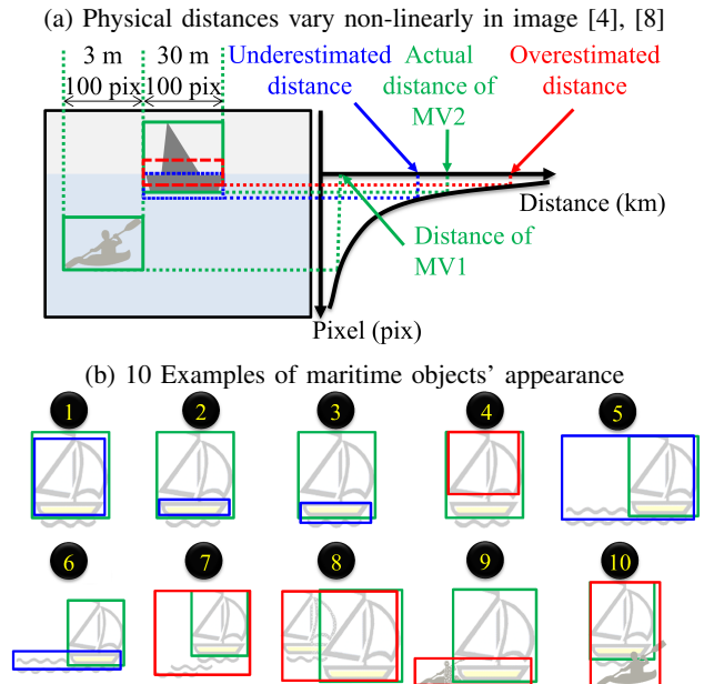
Fig. 1: What is an acceptable detection of a maritime vessel? (a) Collision avoidance requires accurate estimate of the distance, which is related to the bottom edge of the vessel, and the minimum span of a maritime object. (b) Green, blue, and red boxes denote ground truth, acceptable detection, and unacceptable detections, respectively.
