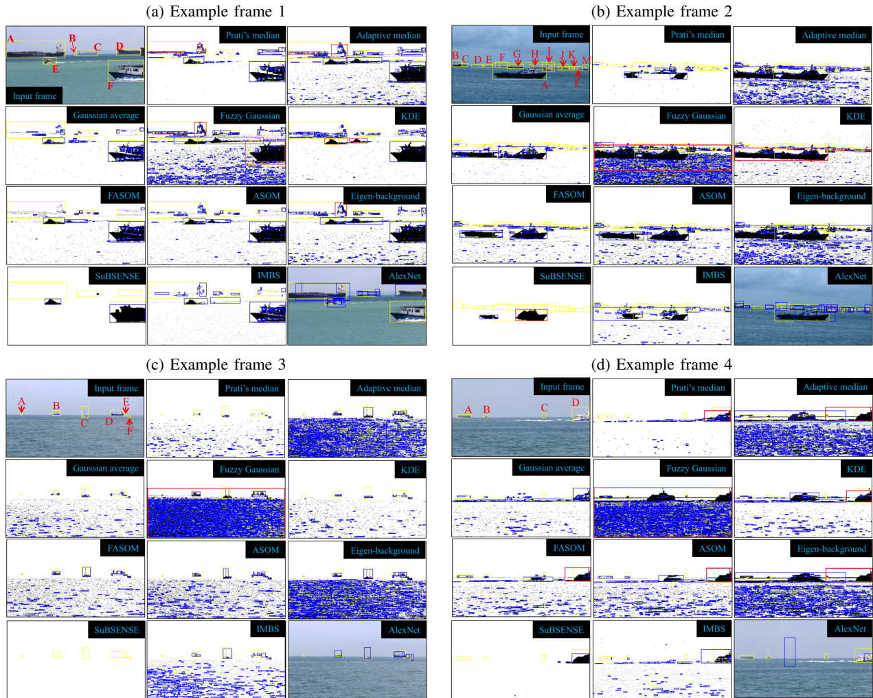
Fig. 6: Example results of CV methods for detection through dynamic BGS. The subtracted background appears white in the results of the methods. Ground truths: yellow BBs. Detected objects (foreground segmentations obtained after BGS): blue or red BBs. Red BBs: DOs referred in the text.
