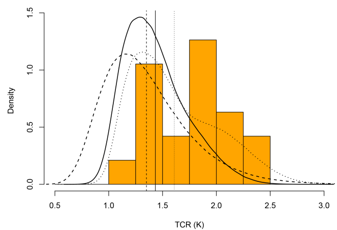
Figure 10. Histogram of the TCR obtained from the different ESMs with the posterior density function estimated from the Monte Carlo simulations using a scale-invariant (solid), a single-exponential (dashed), and a two-exponential (dotted) response function. The vertical lines describe the means of the three approaches.
