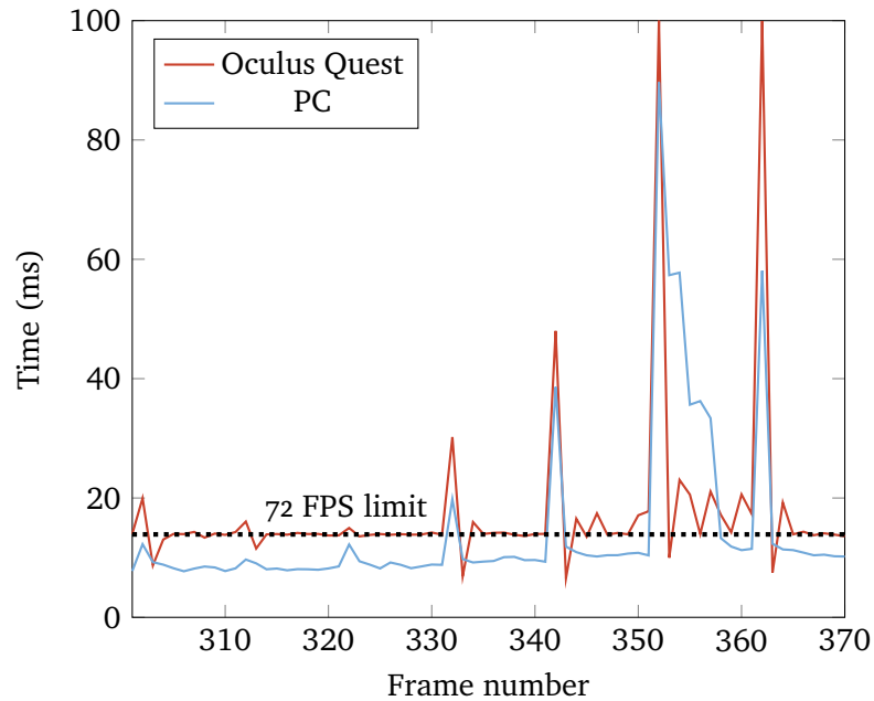
Figure 4.6: Performance of GeneNet VR when visualizing the blood dataset running on a machine and on the Oculus Quest. The x-axis represents the frame number (like a timeline). The y-axis represents the amount of time in milliseconds that a particular frame took to render.
