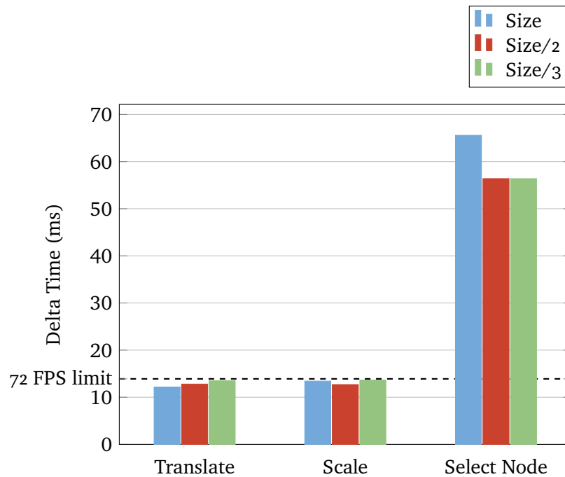
Figure 4.2: Bar graph showing a summary of the performance results for the 1% lowest average (7 frames with worst performance).
