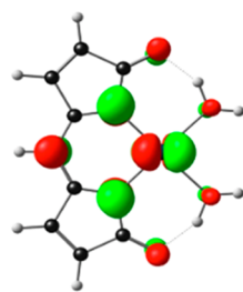
HOMO, b_1
