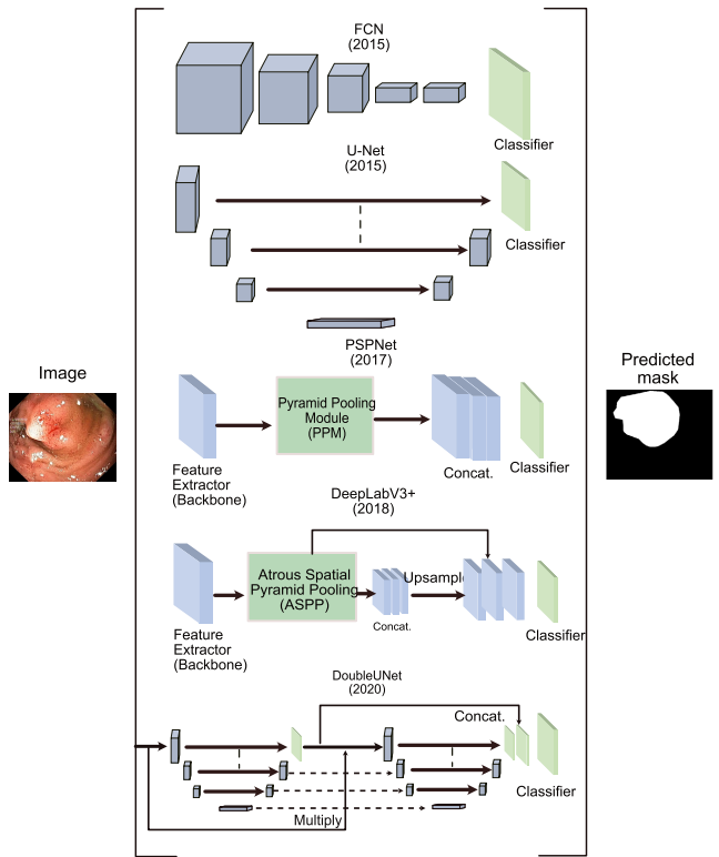
FIGURE 2. Baseline detection, localization and semantic segmentation method summary.
