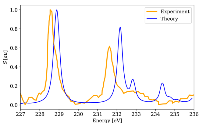
Figure 9. Calculated 4c-DR-TDDFT (PBE0-40HF, VDZ/aVDZ) XAS spectrum near molybdenum M_{4,5} -edges of MoS_4^{2-} and its comparison with the experimental results. 120 The spectra were normalized by setting the maximum to unity. No shift on the energy axis was applied.
