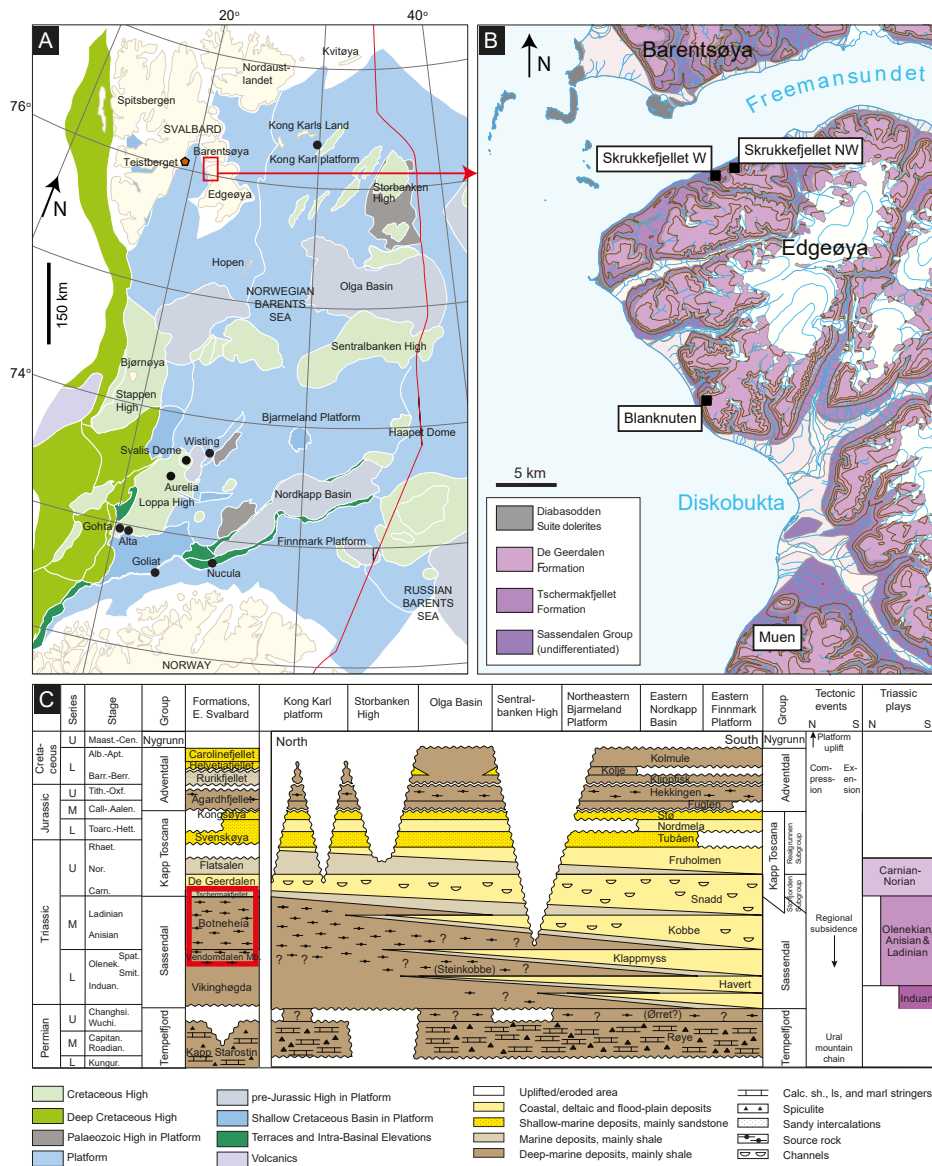
Figure 5.1: (A) Regional map of the Norwegian Barents Sea. The red rectangle marks the study area. The black circles denote fields, discoveries or localities described in the main text. The red pentagon marks the Teistberget locality from which the NGS SR-1 geochemical standard was sampled. Modified from the NPD (2017). (B) Geological map showing the NW part of Edgeøya with the Blanknuten (UTM: 35X E365439 N8664519), Skrukkefjellet W (UTM: 35X E367689 N8682947) and Skrukkefjellet NW (UTM: 35X E369750 N8683650) localities marked. Modified from Dallmann and Elvevold (2015). (C) Regional correlation panel of the Upper Permian to Lower Cretaceous succession from the Finnmark Platform in the south to the eastern islands of Svalbard in the north. Note the diachronous, lateral facies relationship between the Lower–Middle Triassic Steinkobbe Formation and Middle Triassic Botneheia Formation, younging from south to north. Modified from the NPD (2017).
