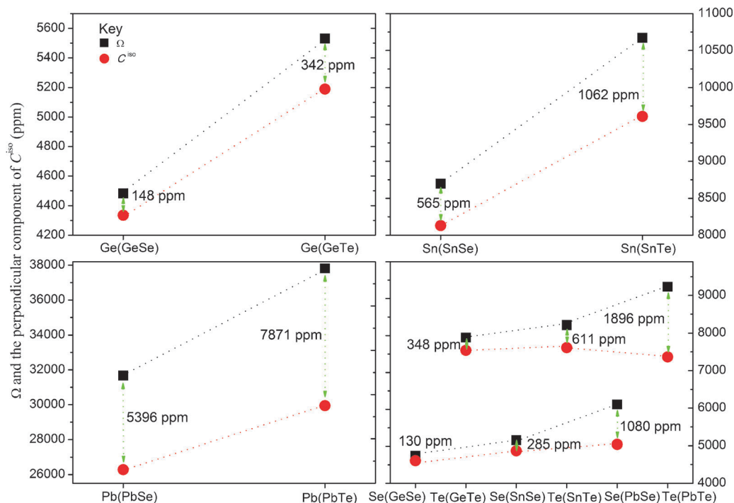
Fig. 2 Comparison of the shielding spans ( \Omega , the squares) and the perpendicular component of the NSR constants ( C_{\perp}^{\text{iso}} , the circles) of XSe and XTe ( X = \text{Ge}, \text{Sn} and \text{Pb} ) molecules: calculated using DKS/BP86/cv4z. The corresponding value for Si in SiSe is 43 ppm, in SiTe is 111 ppm, whereas for Se in SiSe is 74 ppm and for Te in SiTe is 250 ppm.
