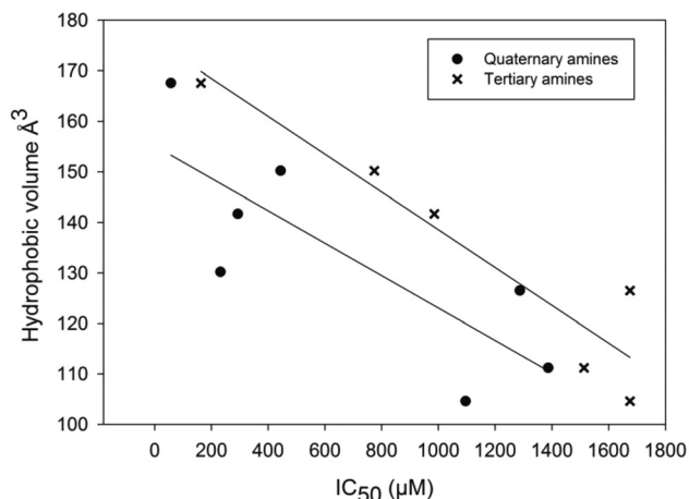
Fig. 3 Correlation plot illustration the influence of the hydrophobic volume on the inhibitory effect of the different types of analogs. -x- are the tertiary amines, 2a–7a and -- represent the quaternary amines 1, 2b–7b.
