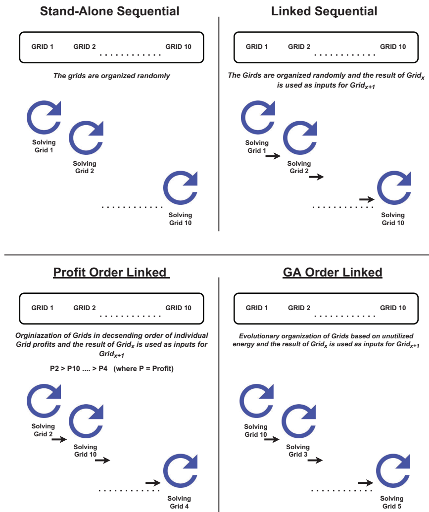
FIGURE 6 Machine chart describing the processes involved in the consensus formations and interactions between grids. Stand-Alone Sequential (top-left), Linked Sequential (top-right), Profit Order Linked (bottom-left), and GA Order Linked (bottom-right)
