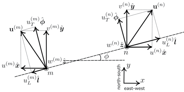
Figure 3. Schematic diagram showing the wind velocity vectors for two different meteor detections n and m on a plane view. The vectors are decomposed in longitudinal, transverse and vertical components u_L , u_T , and w and in Cartesian ENU components u , v , and w . \hat{l} , \hat{\phi} , \hat{z} and \hat{x} , \hat{y} , \hat{z} are the unit vectors of the two systems.
