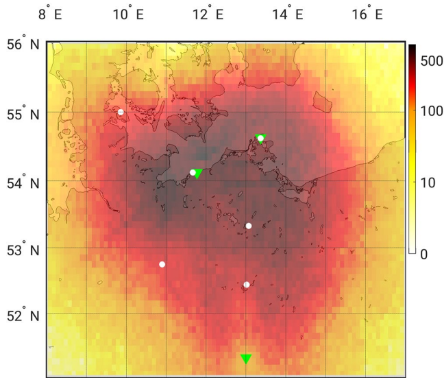
Figure 1. Transmitting and receiving sites during the Spread Spectrum Interferometric Multistatic meteor radar Observing Network (SIMONE) 2018 campaign. The green triangles mark the location of the transmitters and the white circles mark the location with receivers only. The red, orange and yellow tones represent a 2D histogram for the total number of specular meteor observations detected during the campaign. The color bar values show the number of detections within bins of 0.1^\circ wide in Latitude and Longitude.
