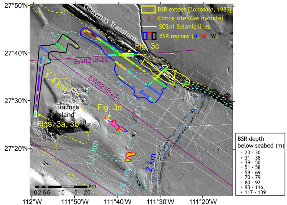
Figure 2. BSR regions and the depth of the BSR below the seafloor. Gas hydrate was recovered from a core in the northern BSR region during the cruise SO241.
