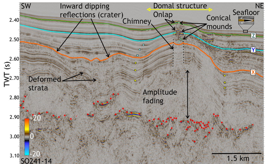
Figure 7. The seismic line (location in Figure 6) showing sill intrusion-related deformation and presence of hydrothermal vent complexes at different stratigraphic levels. Stratal deformation and amplitude blanking are seen in the sedimentary unit overlying the inferred sills (red dots). Conical mounds stack up vertically and are connected by a vertical seismic chimney. The chimney is rooted at the zone of amplitude fading. The zone of amplitude fading is likely due to stratal disruption in the metamorphic aureoles around the sills. Crater and mound-shaped vent complexes occur on reflector X. The axial traces in the fold are near-vertical (small yellow squares) below the reflector X, but they (small cyan squares) dip away from the crest in the overlying layer. The unit bounded between X and Z is deposited above the fold after deformation ceased. They are warped due to differential compaction. The conical mounds are hydrothermal vent complexes formed by the release of hydrothermal fluids on the paleo-seafloor.
