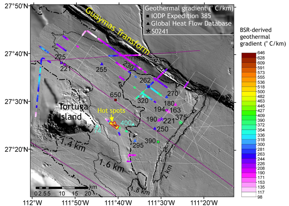
Figure 5. Spatial variations of geothermal gradient derived from the BSR. The red polygon indicates the anomalous hot spots (see also Figure 8b). Geothermal gradients from various surveys and the IODP Expedition 385 are also shown.
