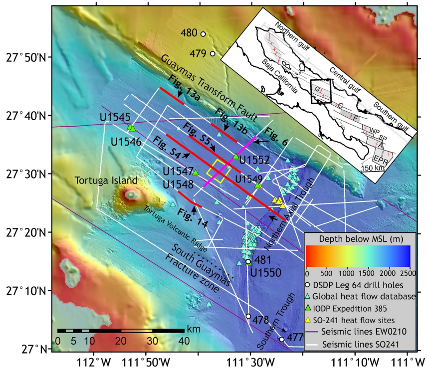
Figure 1. Overview map with bathymetry highlighting the northern and southern Guaymas axial troughs and the transform system. The multibeam bathymetric data is derived from the bathymetric data provided by the UNAM-LUCO group and the bathymetric data acquired during the SO241 cruise. The base map also shows the 2D seismic lines (SO241 and EW0210). Heat flow measurement stations are shown by triangles. The inset shows the major structural elements in the Gulf of California and the location of the Guaymas Basin (after Padilla y Sánchez et al., 2013). Central and southern gulf spreading centers are labeled, G–Guaymas, C–Carmen, F–Farallon, NP–North Pescadero, SP–South Pescadero, A–Alarcon, EPR–East Pacific Rise.
