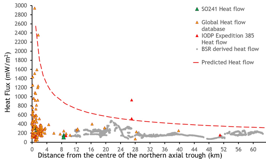
Figure 10. Seafloor heat flow versus distance from the center of the northern axial trough in the northwestern off-axis of the Guaymas Basin. The triangles demarcate the measured heat flow values from the global heat flow database, SO241 heat flow survey, IODP Expedition 385. The gray circles represent the BSR derived heat flow values. The locations of heat flow measurement stations are in Figure 1. The dashed line is the predicted heat flow (Lawver & Williams, 1979).
