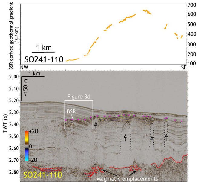
Figure 14. Seismic line showing a convex upward BSR and considerable lateral variation in geothermal gradient. (top) The convex upward geothermal gradient indicates the role of fluid advection. (b) The seismic line shows the magmatic emplacements at 2.65–2.85 s TWT. Several near-vertical zones of amplitude fading (vertical arrows) are inferred as fluid flow conduits that facilitate vertical fluid migration. The shoaling of the BSR could be due to high advective fluxes. The location of the seismic line is shown in Figure 1.
