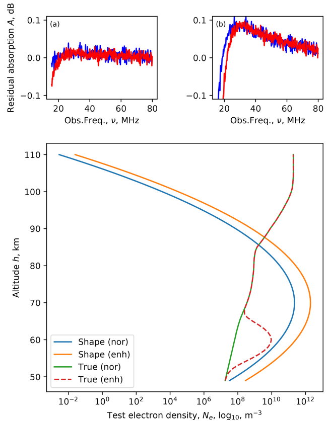
Figure 11. Fitting a 70 km peak Gaussian electron density profile to simulated normal (nor) and enhanced (enh) ionospheric profile data. The residuals are shown in the two top panels as a function of the observing frequency: (a) normal and (b) enhanced, with the o mode shown in blue and the x mode in red.
