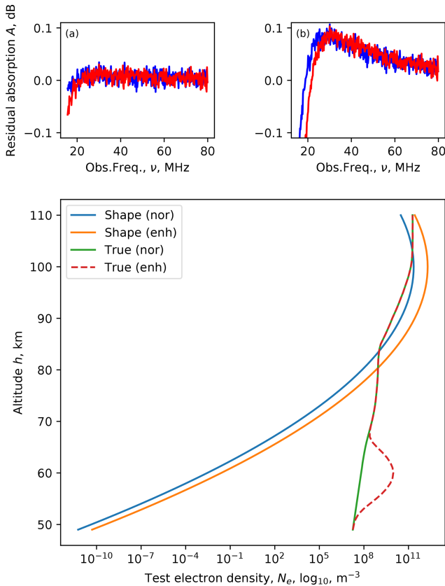
Figure 12. Fitting a 100 km peak Gaussian electron density profile to simulated normal and enhanced ionospheric profile data. The residuals are shown in the two top panels as a function of the observing frequency: (a) normal and (b) enhanced, with the o mode shown in blue and the x mode in red.
