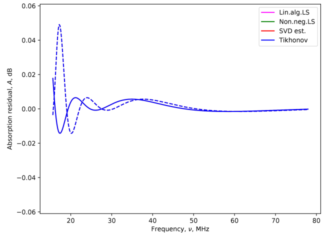
Figure 9. Residuals between data from original and determined models. The solid line corresponds to the o mode, and the dashed line is for the x mode. All four methods give the same result for the given mode. The lines are superimposed, which is why only one colour seemingly appears, even though all methods are being plotted, as per the legend.
