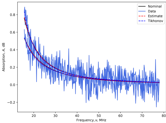
Figure 8. Application of the forward models to different solutions. The black “nominal” line does not readily appear as the “estimate” is collinear with it. The horizontal axis is the observing radio frequency, \nu = \omega/2\pi .
