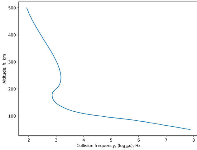
Figure 1. The model of electron collision frequency \nu = \nu_{en} + \nu_{ei} from Aggarwal et al. (1979).
