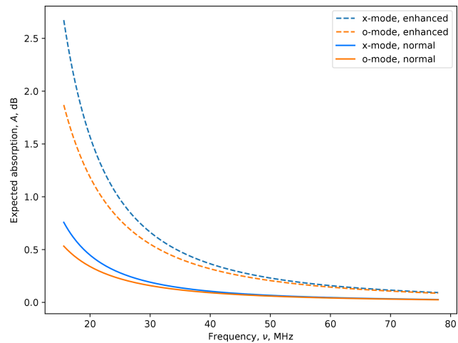
Figure 4. Expected CNA from normal and enhanced conditions for both x -mode and o -mode radio waves. The horizontal axis shows the observing radio frequency, \nu = \omega/2\pi , in megahertz.
