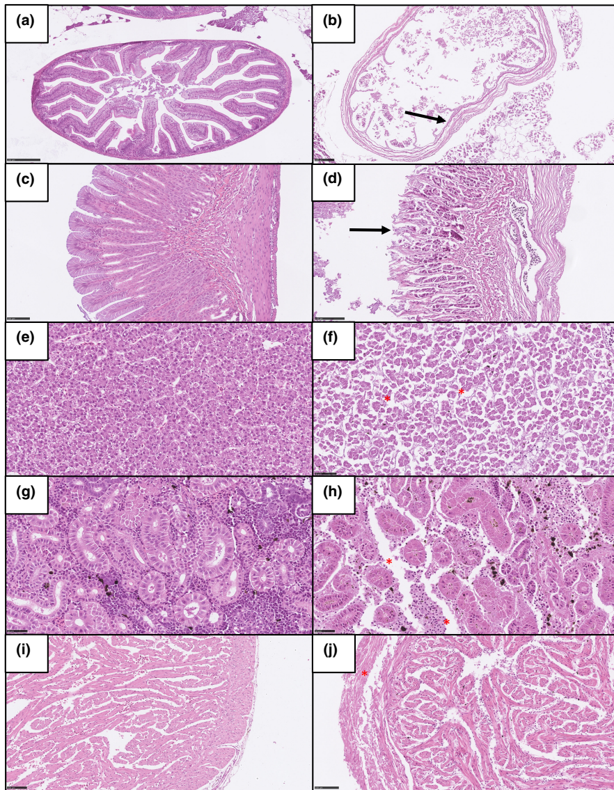
FIGURE 3 Histologic images of different tissues kept at room temperature (RT). Control samples are included for reference. (a) Pyloric caeca and pancreatic tissue, control sample (0 h). (b) Pyloric caeca and pancreatic tissue (24 h), dark arrow shows disintegration and loss of epithelial mucosa. (c) Stomach, control sample (0 h). (d) Stomach (24 h), dark arrow shows disintegration of epithelial cells in gastric mucosa. (e) Liver, control sample (0 h). (f) Liver (24 h), red asterisk (*) shows destruction of liver hepatocytes and sinusoids. (g) Posterior kidney, control sample (0 h). (h) Posterior kidney (24 h), red asterisk (*) shows destruction of kidney, especially the haematopoietic tissue. (i) Heart musculature, control sample (0 h). (j) Heart musculature (24 h), red asterisk (*) shows moderate destruction of cardiac myocytes. Scale bars 50 μm (posterior kidney, liver), 100 μm (heart musculature, stomach and pyloric caeca with pancreatic tissue (24 h)) and 250 μm (pyloric caeca with pancreatic tissue (0 h))
