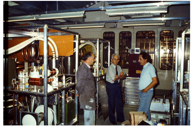
Figure 4. Three important people involved in the construction of Heating. The photograph shows, from left to right, technician Helmut Gegner and scientists Jules Fejer and Helmut Kopka in the transmitter hall in 1979. Four open 100 kW transmitters are visible, which were used in the first experiments. (Photo credit: MPAe)
