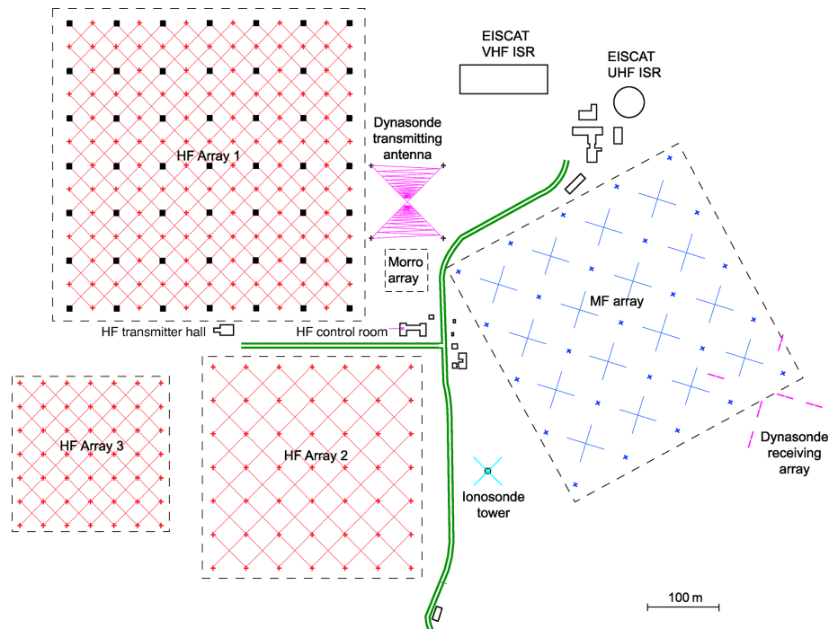
Figure 2. Schematic diagram showing the layout of antennas and major infrastructure at the Ramfjordmoen site (to scale). The red diagonal lines in the HF arrays represent the full-wave antennas attached to wooden masts at each end (small red crosses). The feed points of each crossed-dipole antenna is where the red lines cross each other. The black squares in HF Array 1 show the original 23 m tall wooden masts to which the low-frequency antennas were attached (until 1985), and the red crosses in Array 1 show the 12 m tall wooden masts added around 1989 for the modified array containing higher-frequency antennas similar to Array 3. The Dynasonde (HF sounder), housed in the same building as the HF control room, and its associated antennas are an integral part of the Heating facility. The EISCAT IS radar antennas and buildings are shown at the upper right. The large blue crosses show the crossed half-wave dipoles of the 2.78 MHz MF (medium-frequency) radar transmitting antenna, suspended between masts (small blue crosses). The ionosonde tower supports the transmitting antenna for the University of Tromsø's digisonde. The Morro array is an antenna for a 56 MHz MST (mesosphere–stratosphere–troposphere) radar from the University of Tromsø. The green double line shows the road, and the unlabelled boxes are buildings or huts with optical and other instruments.
