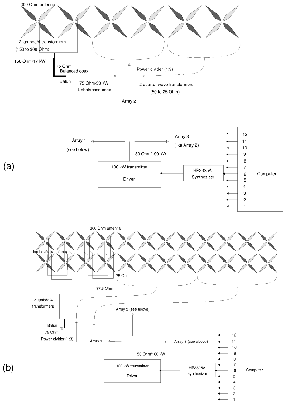
Figure 5. Diagram showing the transmission system and how the power was distributed from one transmitter (a) to six crossed dipoles in each of the antenna arrays before the storm in 1985 and (b) to 24 crossed dipoles in the rebuilt Array 1 from 1990. After 2008, the HP3325A synthesizers were replaced by direct digital synthesizer boards.
