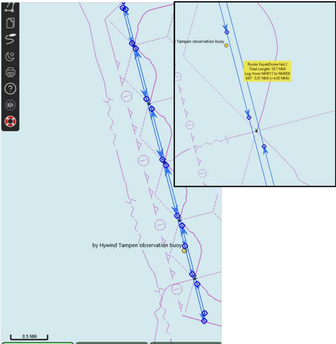
Figure 18. The KayakDrone's acoustic transect, survey design. Where the KayakDrone is to move between and pass by turbine: HY07, HY08, HY09, HY10, and HY11 all standing in one strait line. To the right: A close-up view of the KayakDrone's acoustic transect of the survey design. Blue circles are waypoint where the KayakDrone is repositioning related to the given coordinates in the transect.
