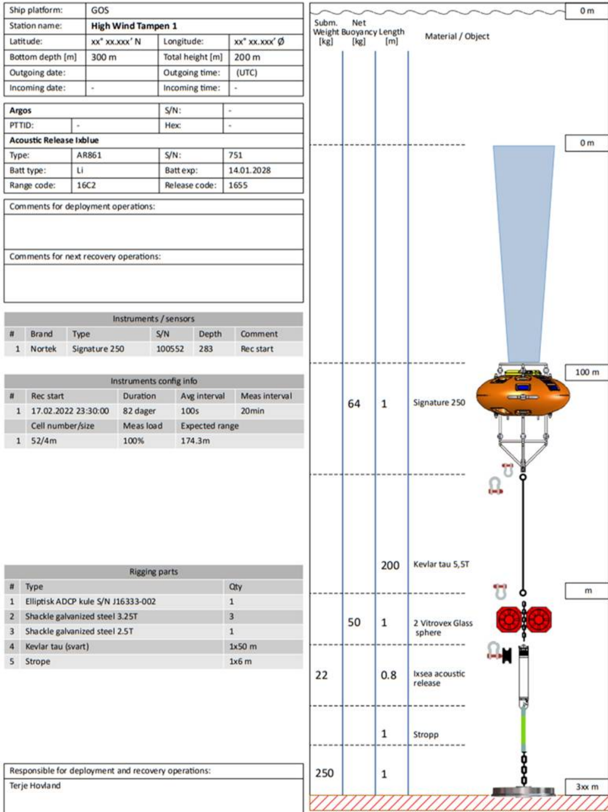
Figure 3. Drawing of the ADCP mooring and instrument information.
