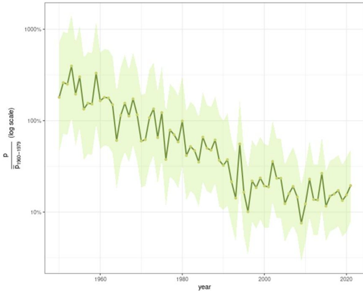
Figure 2.6. Geometric mean of estimated yellow eel recruitment for Europe updated to 2021. The yellow recruitment was estimated using a GLM ( yelloweel \sim year ) fitted to 22 yellow eel time-series p scaled to the 1960-1979 average p_{1960-1979} . Note the logarithmic scale on the y-axis.
