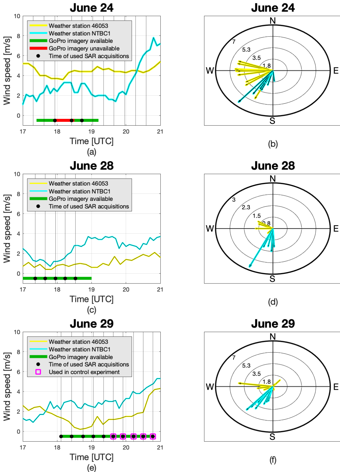
Fig. 5. (a), (c) and (e) show measured wind speed vs. time at the two weather stations shown in Fig. 1. The times of all UAVSAR acquisitions on each day are indicated by the vertical black lines, and the acquisitions used in this analysis are indicated with black dots. The purple boxes indicate acquisitions that are used in the control experiment. The time extents of the GoPro imagery are indicated by the horizontal green (available) and red (unavailable) lines. (b), (d) and (f) show the direction the wind came from, measured at the times of all UAVSAR acquisitions. The concentric circles indicate the magnitude of the wind speed in m/s.
