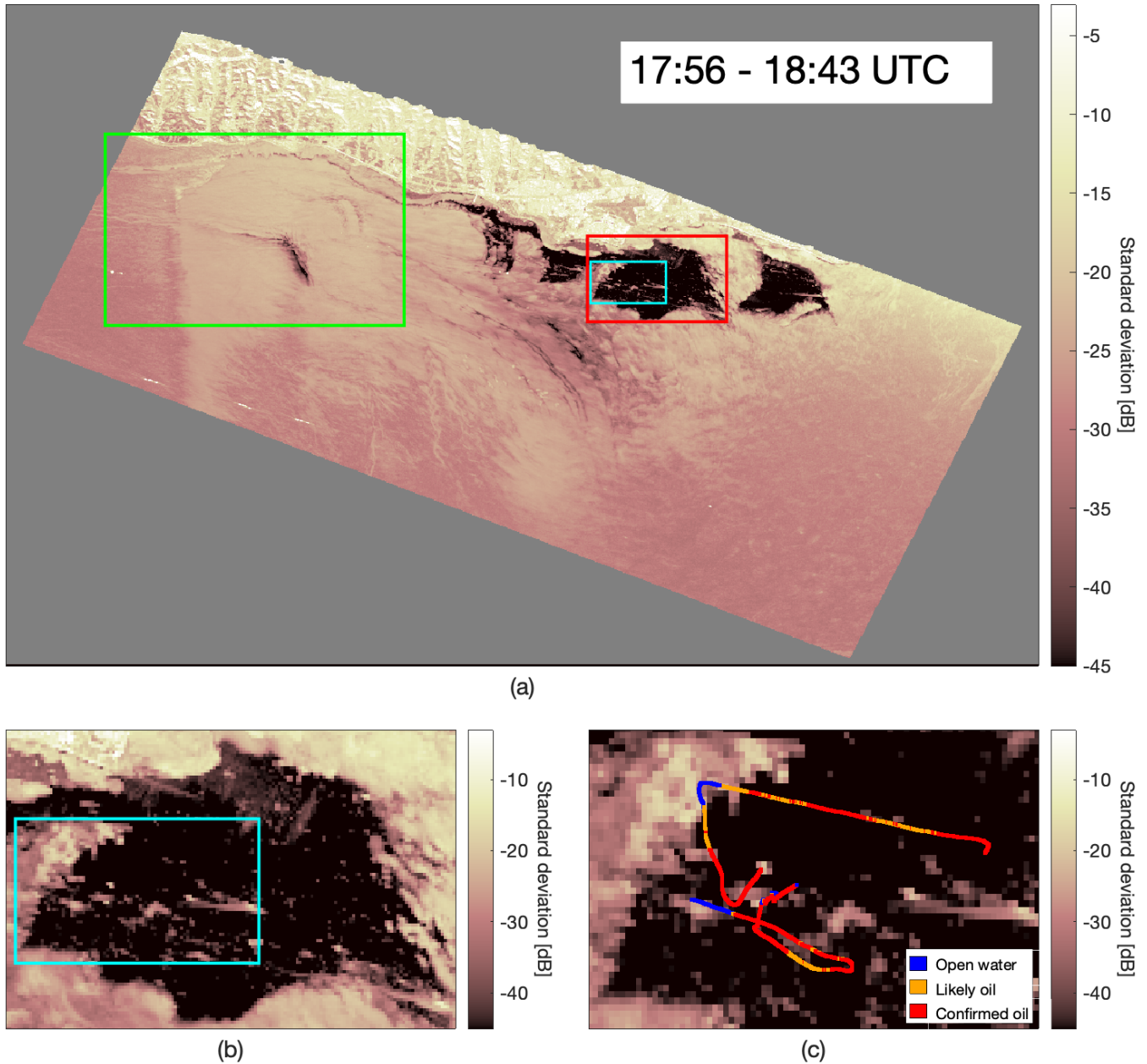
Fig. 11. (a) High confidence oil/open water map for June 24, 2022, based on scenes 2-4. The low values (plotted as dark areas) are likely mineral oil slicks while the high values (plotted as bright areas) are likely open (unslicked) water. (b) The area that corresponds to the red ROI in (a) is shown and the oil slick is a clearly delineated dark region with sharp borders. (c) The map for the smaller cyan ROI in (b) is shown as well as a classified boat track. Time extent for classified GoPro imagery is 17:26 – 19:13 UTC (SAR imaging time \pm 30 minutes).
