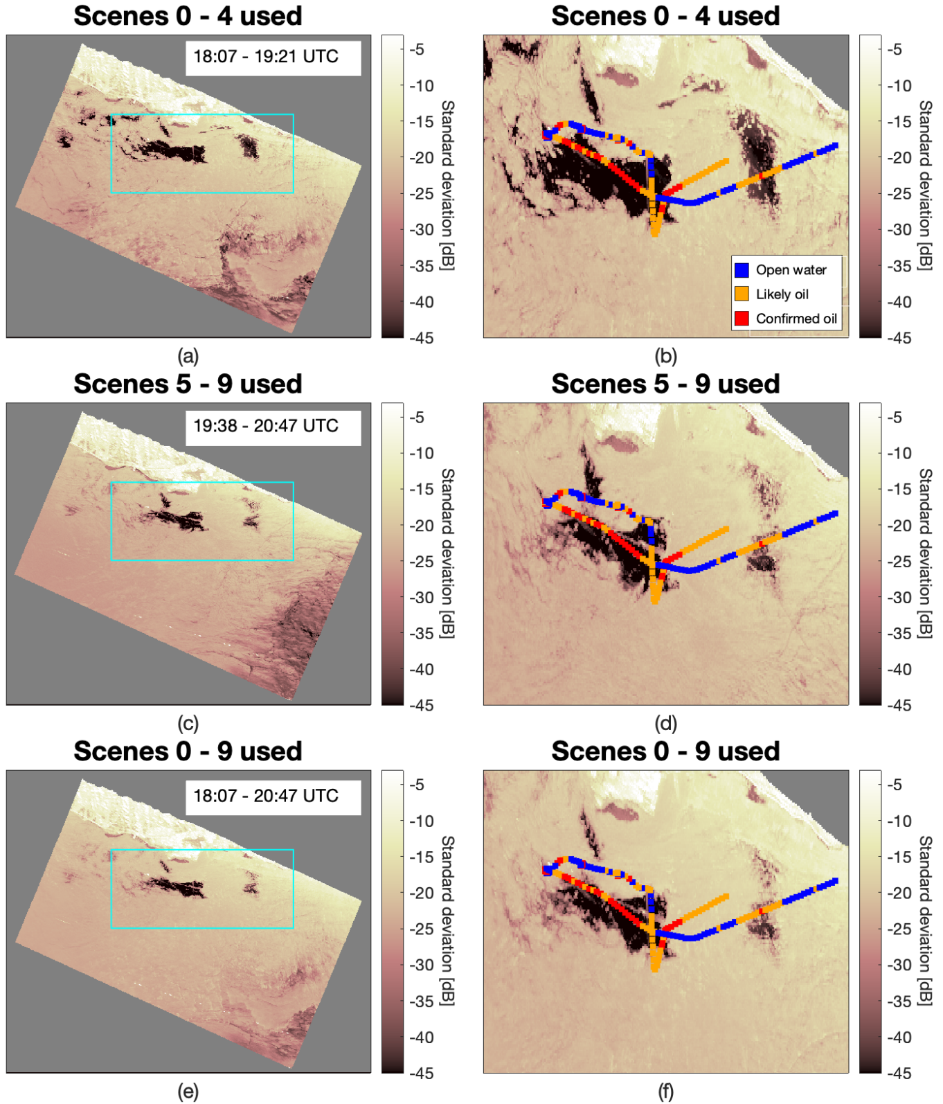
Fig. 16. June 29 high confidence oil/open water maps for instances when (a) the first five scenes of the time-series are used, (c) the last five scenes of the time-series are used and (e) all ten scenes in the time-series are used. The cyan box is a ROI that outlines an area of what is believed to be mineral oil over which the boat traversed. (b), (d) and (f) show the cyan ROI from (a), (c) and (e) respectively. The classified GoPro imagery track is overlaid on these images and displayed in red, orange, and blue for the different classes. Time extent for classified GoPro imagery is 18:07 – 20:47 UTC.
