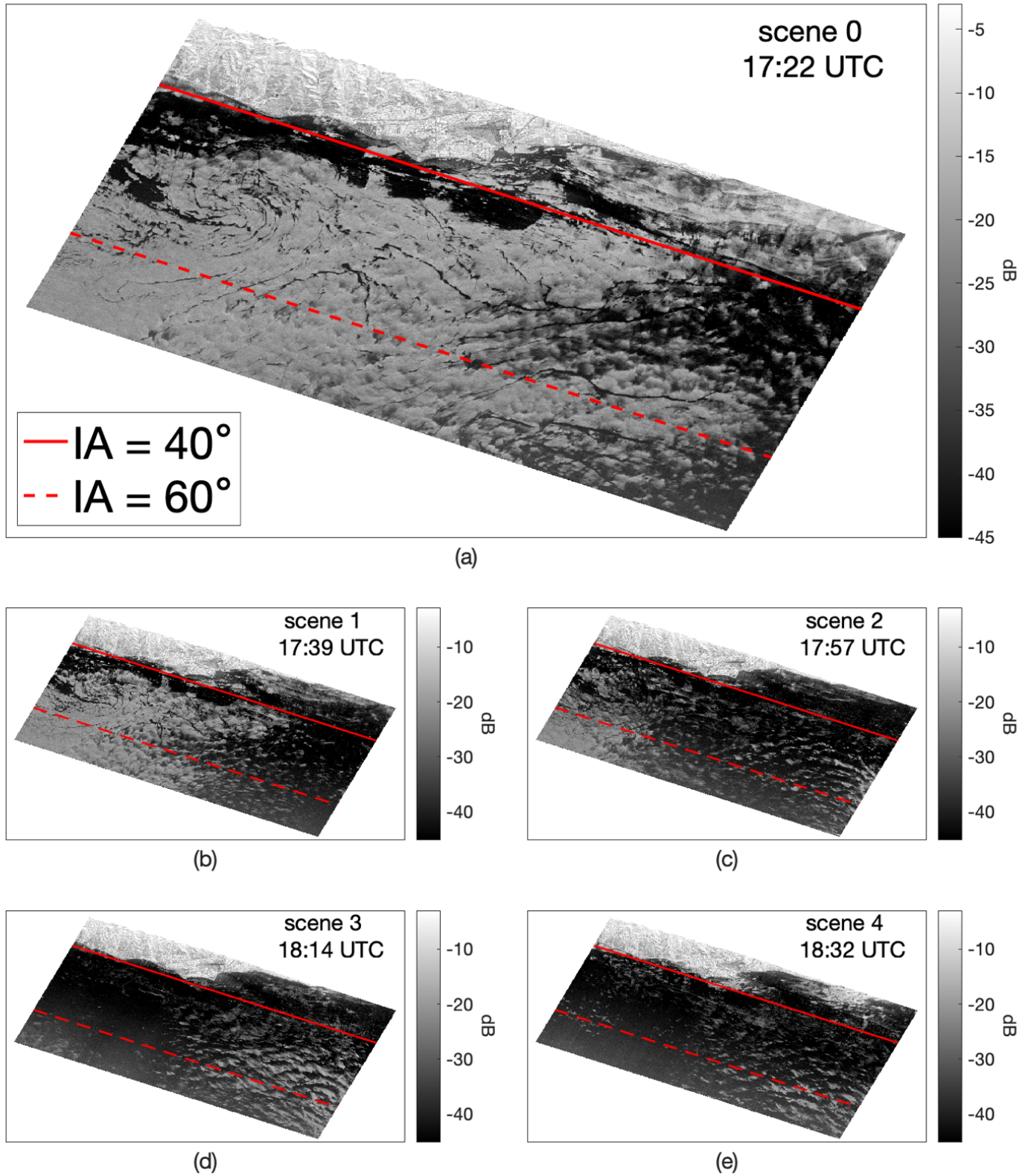
Fig. 3. (a) – (e) VV-intensity images for all scenes acquired on June 28, 2022. Scenes contain areas of both oil slick and low wind. The low wind zones cover most of the image in (c) – (e).
