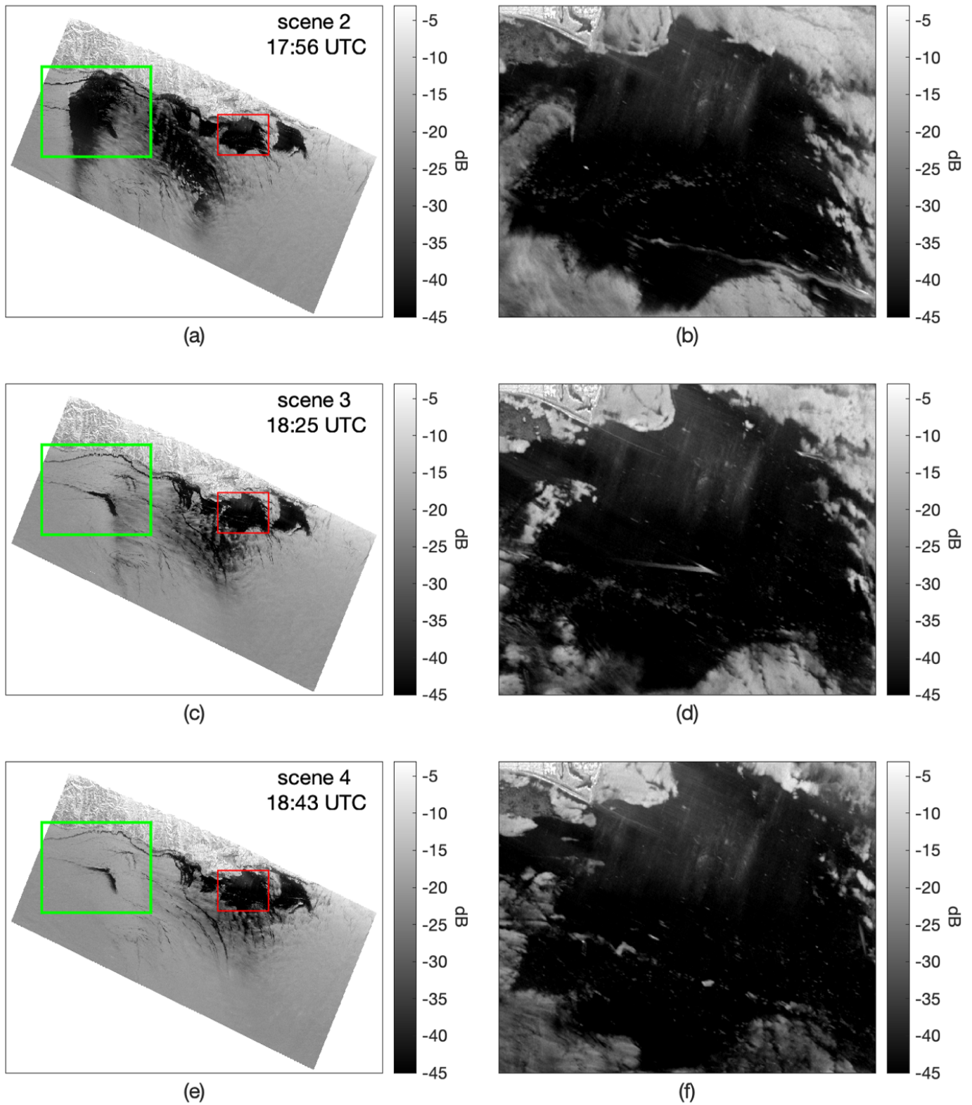
Fig. 2. (a), (c) and (e) VV-intensity images for scenes 2, 3 and 4 acquired on June 24, 2022. An area of low wind, indicated by a radar dark patch, can be seen traversing the imagery from the far left/middle of the scene to the right side of the scene throughout the time-series. The red region of interest (ROI) shows where the boat was during the times these scenes were acquired. Two streamers are outlined by the green ROI. (b), (d) and (f) are zoomed-in on the red ROI in (a), (c) and (e), respectively.
