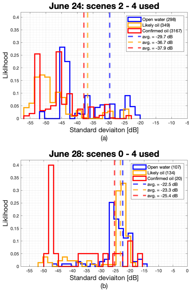
Fig. 12. Histograms of standard deviation values that correspond to the GoPro tracks for June 24 and June 28 separated by class. Number of GoPro images sorted into each class indicted in parentheses in the legend.
