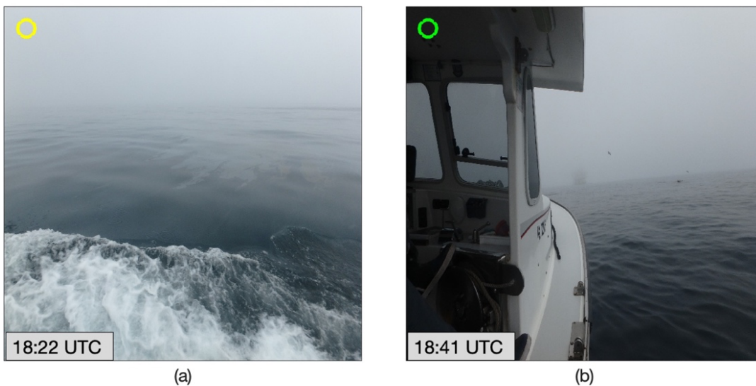
Fig. 9. Photographs taken from the boat with a handheld camera. (a) The boat is in an area of thin oil, where the boundary of a thicker oil region is a short distance away. Glare obscures any features or color discontinuities of the slickened surface. (b) Boat is in an area of open water. Due to low wind and effect of fog, small surface ripples (indicative of open water) are more difficult to observe. The position of the photos in Fig. 13 are marked with the corresponding yellow and green circles.
