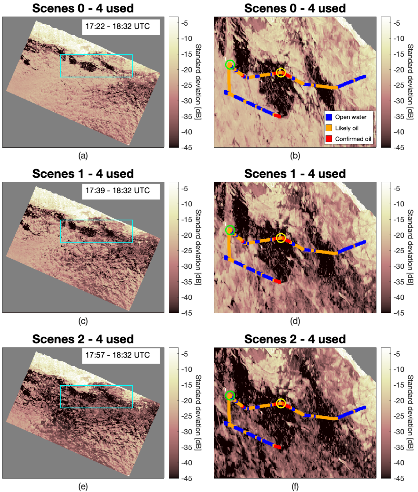
Fig. 13. June 28 high confidence oil/open water maps for instances when (a) all five scenes of the time-series are used, (c) the first scene was excluded, and (e) the first two scenes were excluded. The cyan box is a ROI that outlines an area where the boat traversed in which mineral oil slicks were present. (b), (d) and (f) show the cyan ROI from (a), (c) and (e), respectively with classified GoPro imagery tracks. Time extent for classified GoPro imagery is 16:52 – 19:02 UTC (SAR imaging time \pm 30 minutes). The green and yellow circles indicate locations where the handheld photographs in Fig. 9 were taken.
