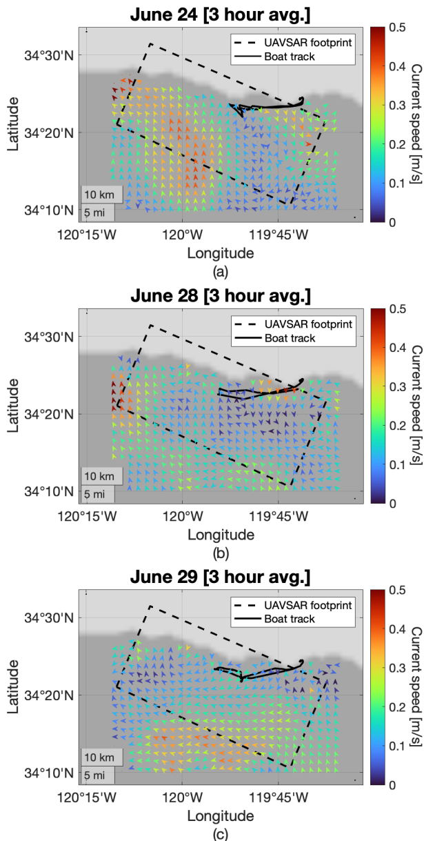
Fig. 6. Average surface current velocity at 2 km resolution from shore-based HF radars, measured over a period of 3 hours corresponding to the acquisition time of the UAVSAR. The UAVSAR swath (dashed line) and the boat tracks (solid black lines) are indicated.
