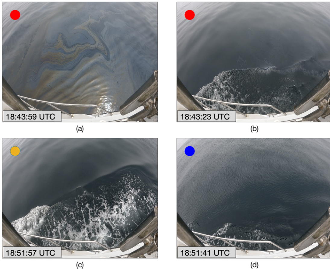
Fig. 8. Examples of classified GoPro images. (a) GoPro images with clearly visible oil is classified as confirmed oil and indicated with a red label. (b) A smooth, featureless surface with some indications of oil is also classified as confirmed (red), here seen as silver sheen in the very center of the image. (c) Smooth featureless surface with no other indications of oil is classified as likely oil, indicated by an orange label. (d) When small surface ripples characteristic of undamped capillary waves is observed, a blue label is applied indicating open water.
