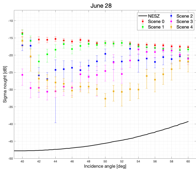
Fig. 14. Mean \sigma^0 values, \pm 1 standard deviation (vertical bars), for the backscatter in the 95 th to 99 th percentile, for each incidence angle bin between 40° and 60° for the 5 scenes in the June 28 time-series. All mean values are at least 10 dB above the UAVSAR NESZ, shown in black.
