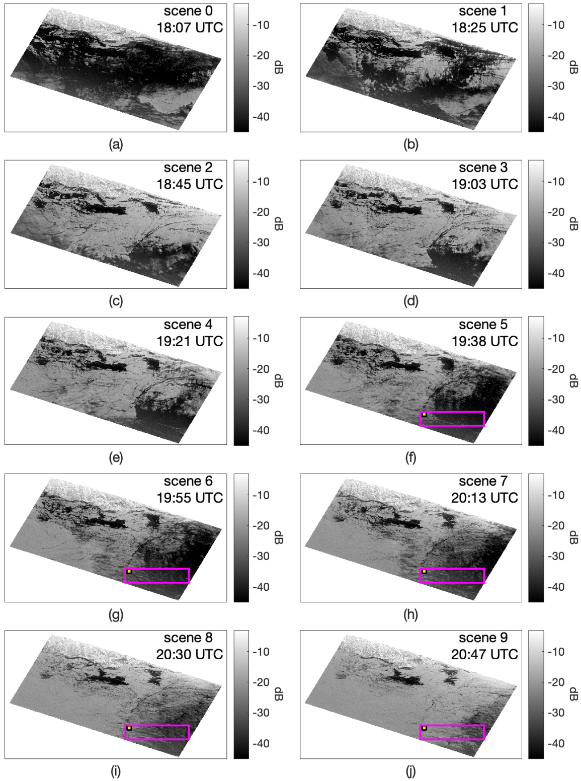
Fig. 4. (a) - (j) VV-intensity images for all scenes acquired on June 29, 2022. Scenes contain areas of both oil slick and low wind. The 46053 weather buoy is marked by the yellow point. The purple rectangle outlines an area far from the seep field containing radar dark zones believed to solely be areas of low wind. This area is used in the control experiment (Section IV C).
