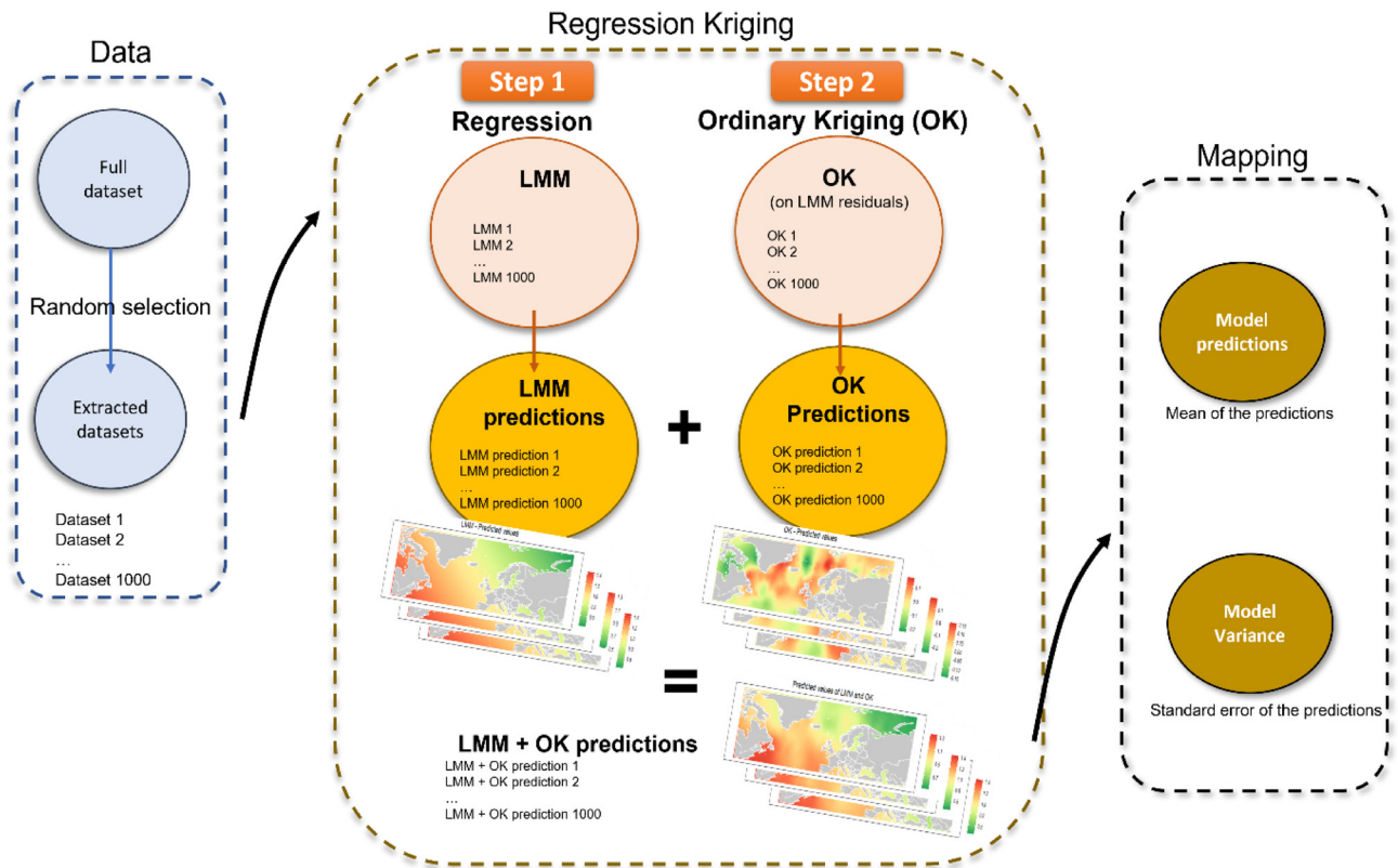
Fig. 2. Schematic description of the statistical analyses with 1) data preparation, 2) regression kriging with step 1 (regression) and step 2 (ordinary kriging), and 3) mapping of model predictions (estimated Hg concentrations).
