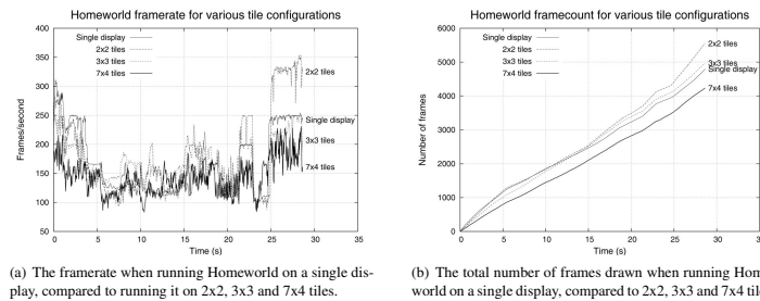
Figure 10: Homeworld performance measurements.
