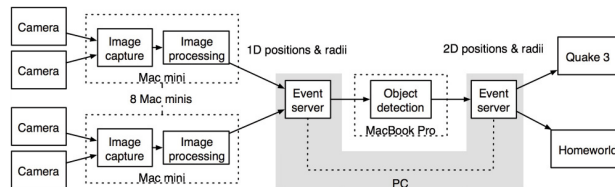
Figure 5: The architecture of the touch-free interface.
