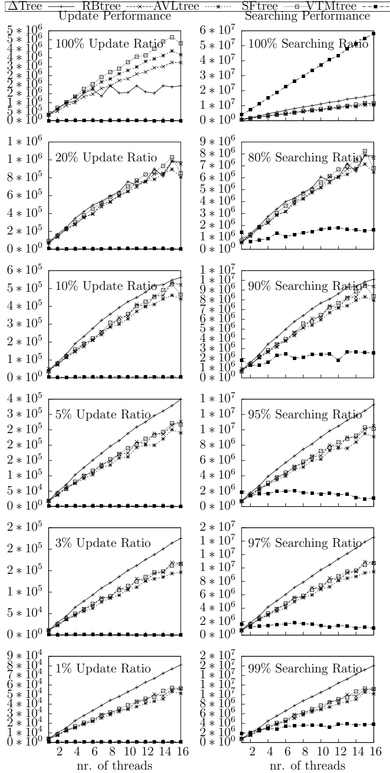
Figure 12: Performance rate (operations/second) of a \Delta Tree with 2,500,000 initial members. The y-axis indicates the rate of operations/second.
