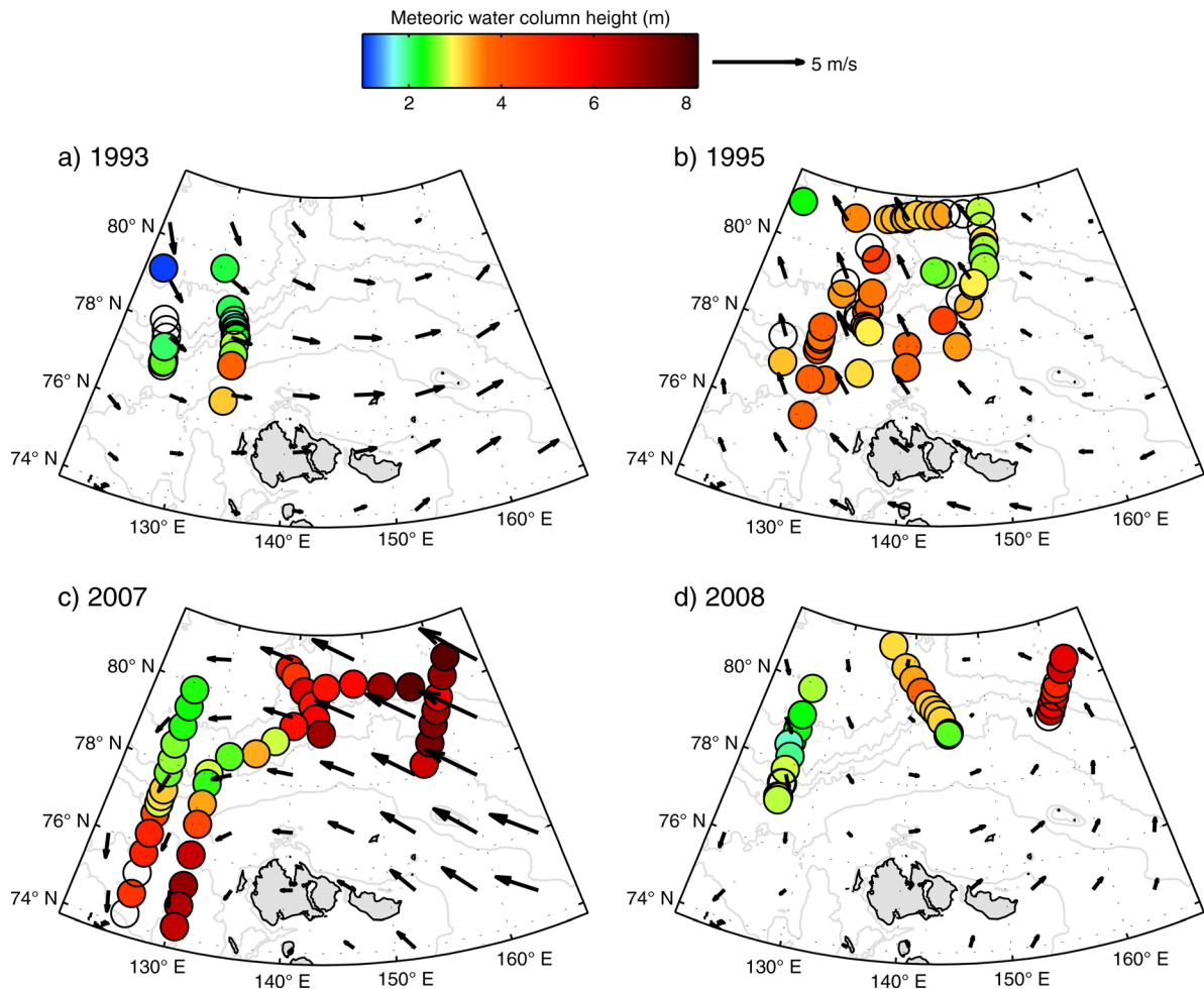
FIG. 12. Maps showing the integrated (0–50 m) water mass fractions for meteoric water in 1993, 1995, 2007, and 2008. From Abrahamsen et al. (2009), updated.
