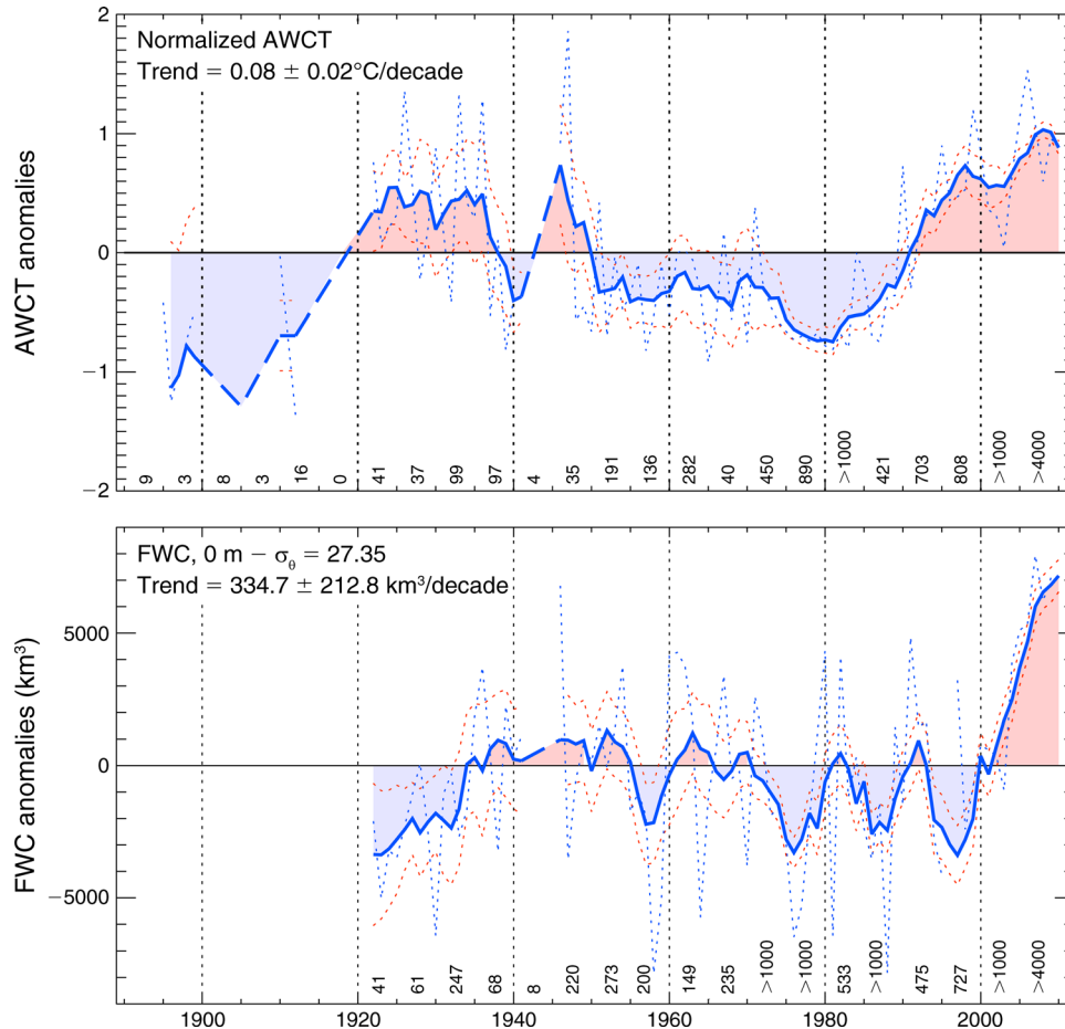
FIG. 6. The Arctic Ocean normalized AW core temperature (AWCT) anomalies and upper \sigma_{\theta} layer (water layer between isopycnals [surfaces of equal density]) FWC anomalies ( \text{km}^3 ). Annual anomalies are shown by blue dotted lines, 7-yr running means are shown by blue thick lines (dashed segments represent gaps in the records), and red dotted lines show their confidence intervals defined by standard errors. Numbers at the bottom denote the 5-yr averaged number of stations used in the data analysis.
