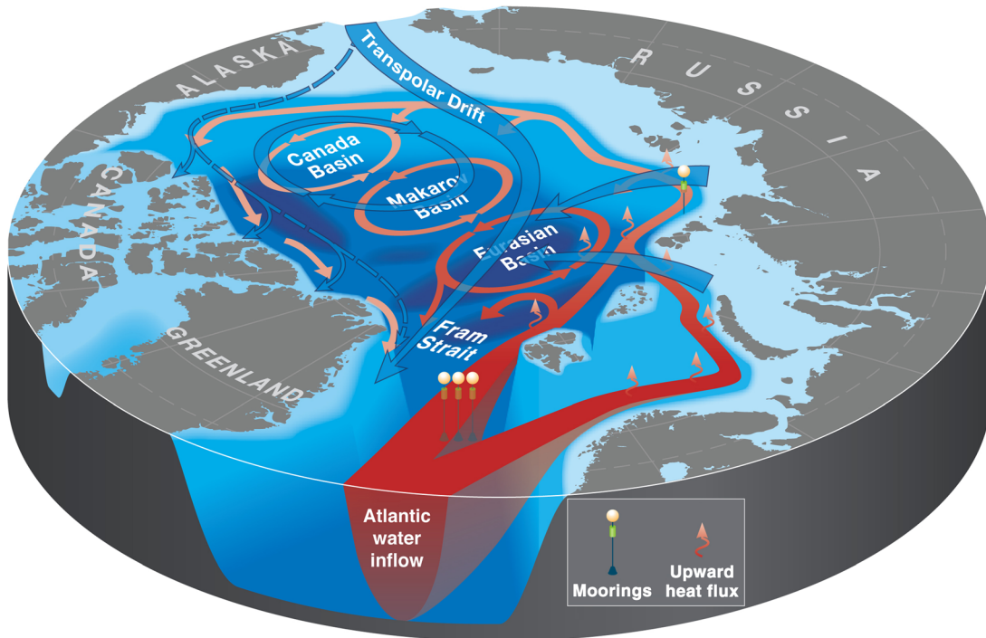
FIG. 3. Circulation of the surface water (blue) and intermediate Atlantic water (red) of the Arctic Ocean. Moorings are autonomous devices moored to the seafloor and measuring various water parameters.
