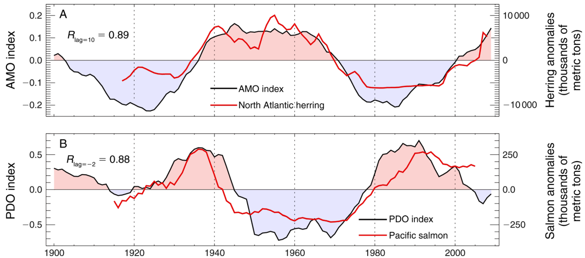
FIG. 2. Time series of major climatological indices: (A) Atlantic Multidecadal Oscillation (AMO; black line) and (B) Pacific Decadal Oscillation (PDO; black line). Also shown are (A) lagged North Atlantic spring-spawning herring biomass anomalies (Toresen and Ostvedt 2000; red line) and (B) Pacific salmon total catch anomalies (Klyashtorin and Lyubushin 2007; red line).
