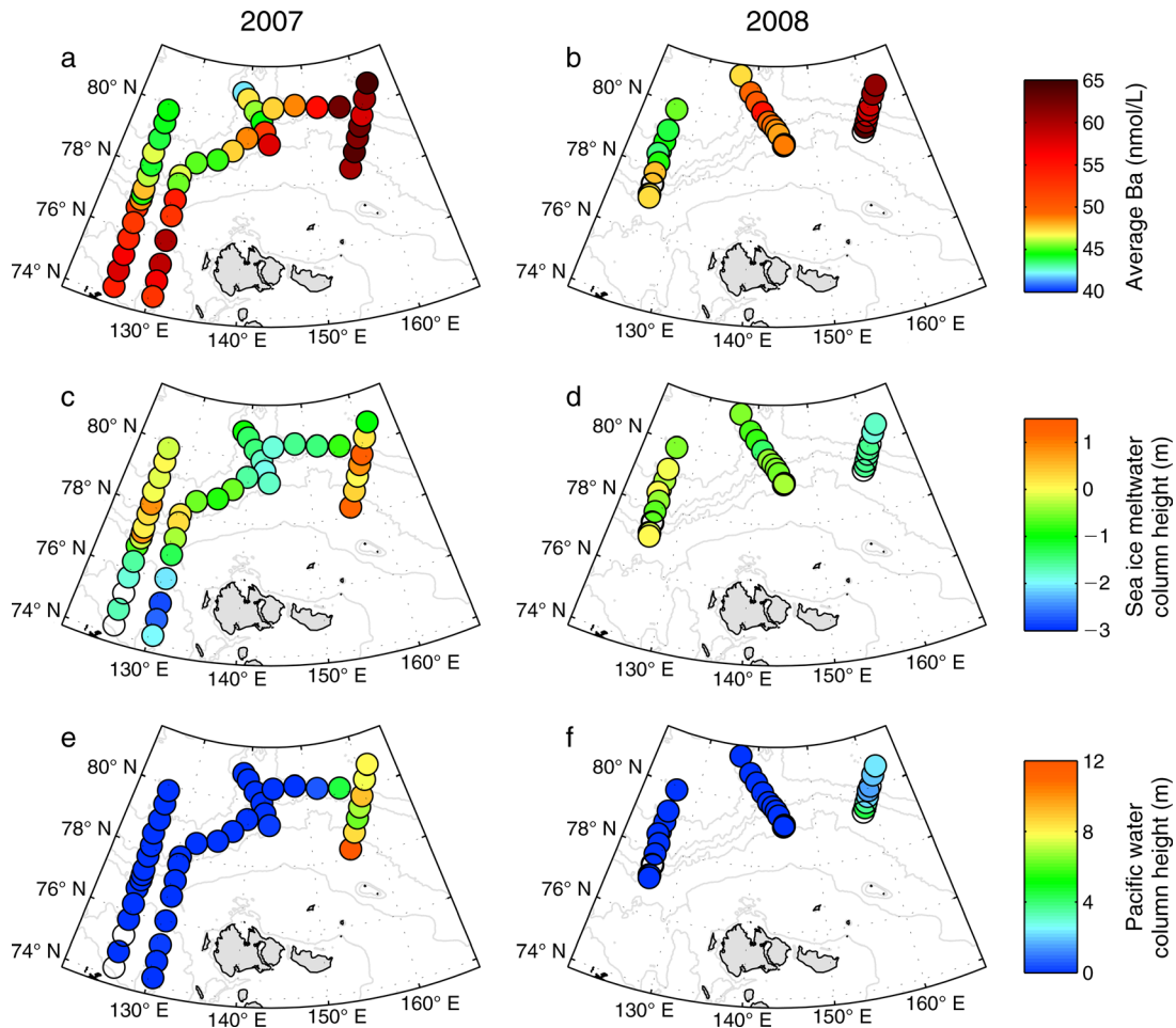
FIG. 13. (a, b) Average dissolved barium concentration, (c, d) integrated water mass fractions for sea-ice melt, and (e, f) integrated water mass fractions for the Pacific water. All of these plots are integrated or averaged from the surface to 50 m depth. The figure is from Abrahamsen et al. (2009), updated.
