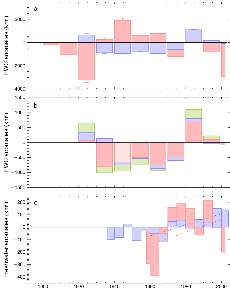
FIG. 11. (a) Decadal (except for the last two years) FWC anomalies and their standard errors for the central Arctic Ocean (red) and Greenland and Barents seas (blue). (b) Decadal FWC anomalies for the Siberian marginal (green), Barents (blue), and Greenland (red) seas. (c) Pentadal freshwater input anomalies of the difference between precipitation and evaporation over the Arctic Ocean (red) and river discharge (blue; adopted from Peterson et al. [2006]). Linear trends over 1955–2002 are shown by dotted lines. Positive anomalies represent fresher basin or input leading to freshening . This figure suggests that the FWC anomalies generated on arctic shelves (including anomalies resulting from river discharge inputs) and those caused by net atmospheric precipitation were too small to trigger long-term FWC variations in the central Arctic Ocean; to the contrary, they tend to moderate the observed long-term central-basin FWC changes. The figure is from Polyakov et al. (2008).
