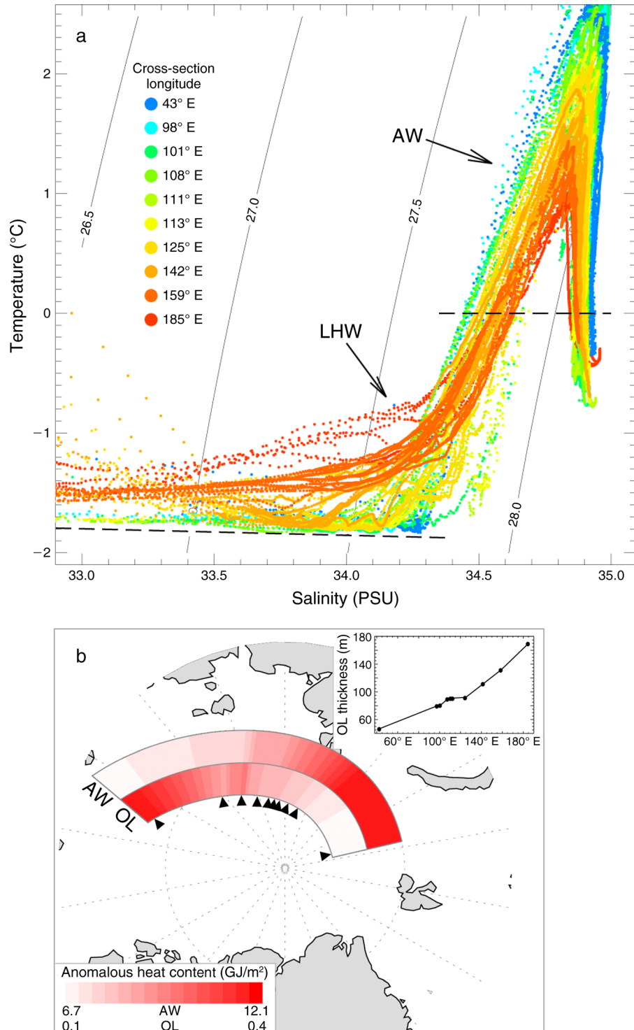
FIG. 10. (a) Potential temperature–salinity plot for the 10 cross-sections carried out in 2007. All temperature and salinity profiles for each cross-section are shown. At low salinities ( <34.3 psu), temperatures are substantially higher at eastern sections (orange) compared with western sections (green). Water masses shown are lower-halocline water (LHW) and Atlantic water (AW). Isolines show potential densities. (b) Anomalous heat content ( \text{GJ/m}^2 ) in the AW and overlying (OL) layers. Black triangles show positions of cross-sections that provided observational data; linear interpolation is used in between. The insert shows along-slope OL thickness change. These two panels provide evidence of the upward spread of AW heat along the AW path in the basin interior. The figure is from Polyakov et al. (2010).
