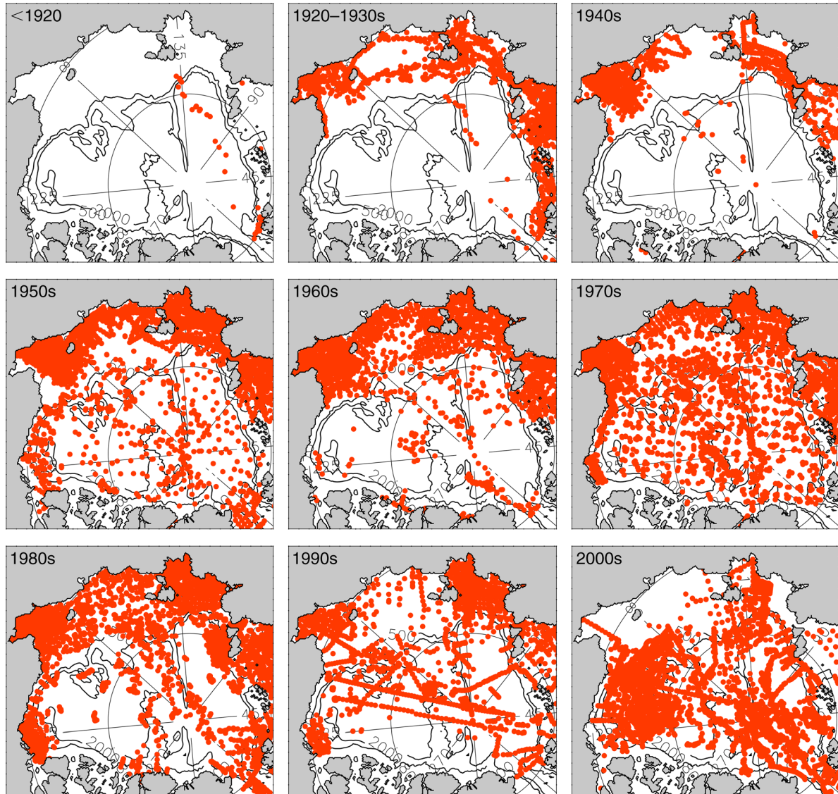
FIG. 5. Maps of the Arctic Ocean showing the locations of deep-basin and shelf oceanographic stations used in this study (red dots).
