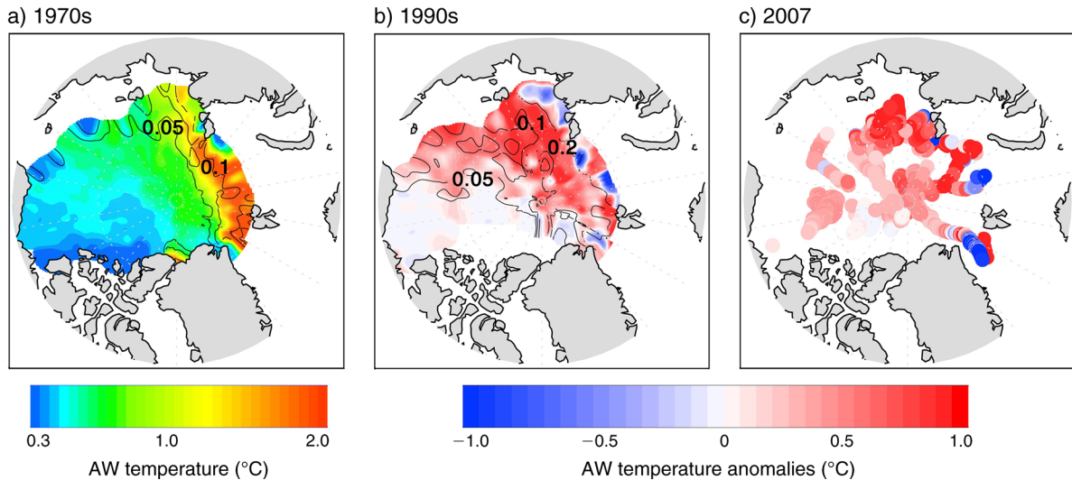
FIG. 7. (a) Mean AW temperature averaged over the 1970s; (b, c) AW temperature anomalies averaged over the 1990s and for data from 2007. Anomalies are computed relative to climatology shown in panel (a). Isolines 0.05, 0.1, and 0.2 in panels (a) and (b) show standard errors (°C); they are small ( <0.05^{\circ}\text{C} ) in the Canada Basin and higher, up to 0.1^{\circ}\text{C} , at some places 0.2^{\circ}\text{C} , in the Eurasian Basin.
