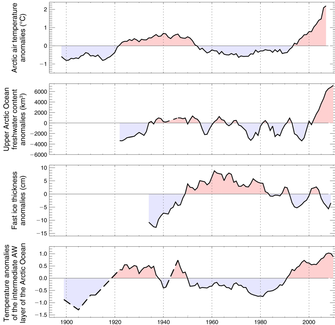
FIG. 1. Comparative long-term evolution of key components of the Arctic climate system. Composite time series of 7-year running mean anomalies of (from top to bottom) the Arctic surface air temperature (Bekryaev et al. 2010), upper 150-m Arctic Ocean freshwater content (FWC; fresher Arctic Ocean is associated with positive FWC anomalies [Polyakov et al. 2008]), composite (15 stations) fast ice (motionless seasonal sea ice anchored to the sea floor and/or the shore that melts and reforms each year) thickness anomalies, and normalized intermediate Atlantic water (AW) core temperature of the Arctic Ocean (Polyakov et al. 2004; values are standard deviations). All records are updated using data from the 2000s. Broken lines are used to indicate gaps in data where we used linear interpolation.
