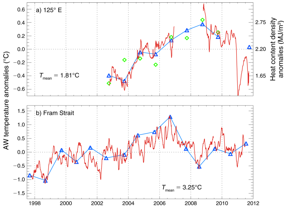
FIG. 8. Time series of AW temperature anomalies ( ^{\circ}\text{C} ) relative to the time-series means from oceanographic sections [blue; mean temperatures T_{\text{mean}} shown on panels], mooring observations [red; panel (a) depth = 260 m, panel (b) depth = 250 m], and heat content density of the layer overlying the AW [green; \sim 50 –125 m depth range, \text{MJ}/\text{m}^3 ]. The mooring records were de-seasoned; conductivity, temperature, and depth (CTD) data are collected in summer so that the seasonal signal does not preclude meaningful interpretation of CTD records. The figure is from Polyakov et al. (2011), updated with 2009–2011 data.
