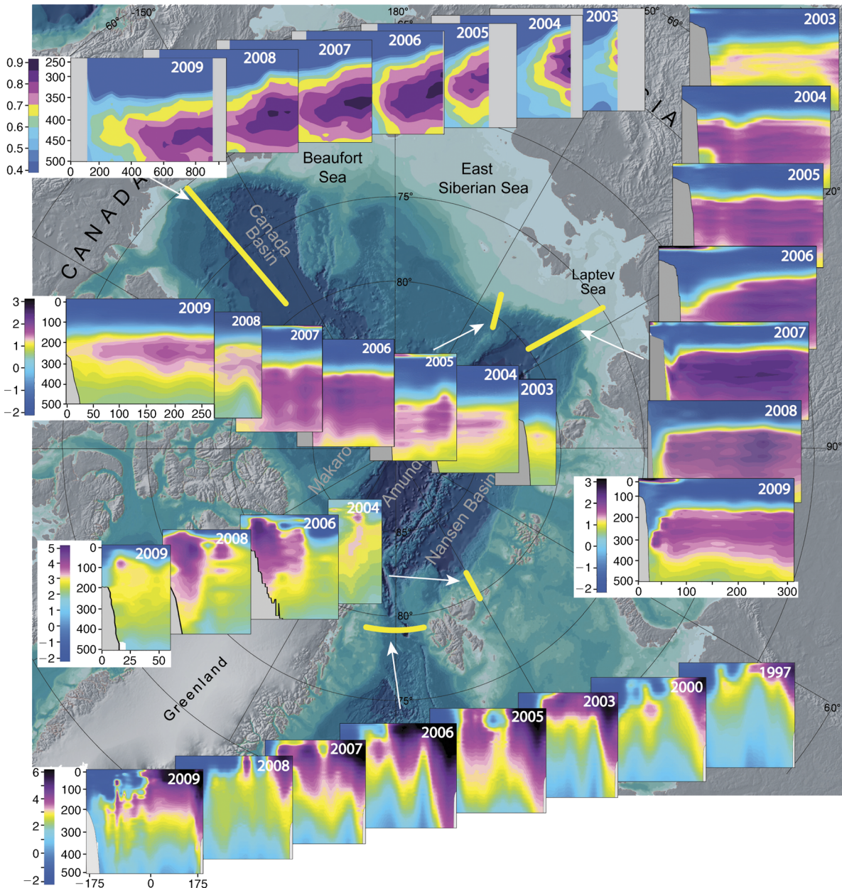
FIG. 9. Vertical cross-sections of water temperature from the Arctic Ocean. The five series of cascaded plots show temperatures measured at the five locations shown by yellow lines on the map. In each set, the x -axis shows distance from the southern end of the section (km), and the y -axis shows depth (m). The scale to the left of the y -axis shows water temperature ( ^{\circ}\text{C} ). Note that the horizontal scale and temperature scale vary from one cascaded set to another. Warming in the Eurasian Basin, approximately in the center of this figure, is associated with the warm AW pulse, which was found in Fram Strait, the gateway to the Arctic Ocean, east of Greenland, in 1999. This pulse peaked in the Eurasian Basin in 2007–2008. In contrast, the warm anomaly in the Canada Basin is related to an earlier pulse of warm water, which entered the Arctic Ocean interior through Fram Strait in the early 1990s. Note that not all available sections are shown for the Fram Strait region. The figure is from Polyakov et al. (2011).
