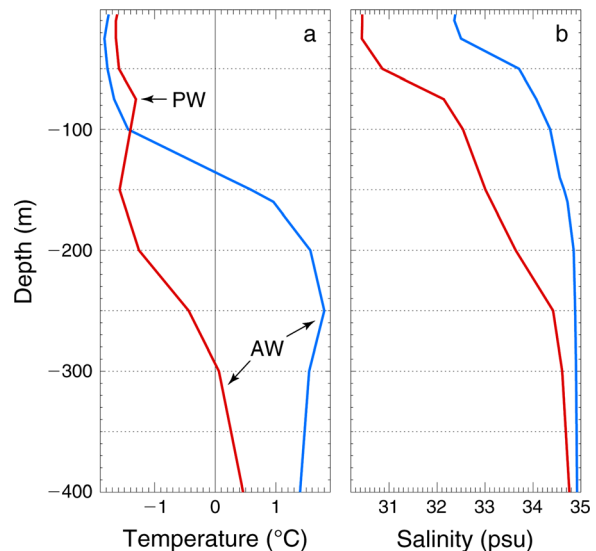
FIG. 4. Vertical profiles of (a) water temperature and (b) salinity collected in the Eurasian Basin (blue; 84.37^\circ N, 80.00^\circ E) and Canadian Basin (red; 80.25^\circ E, 97.60^\circ W) in 1974 showing Arctic Ocean water mass structure. Intermediate AW is identified by water temperatures >0^\circ\text{C} whereas Pacific water (PW) is associated with the temperature maximum above the AW layer and below the upper mixed layer.
