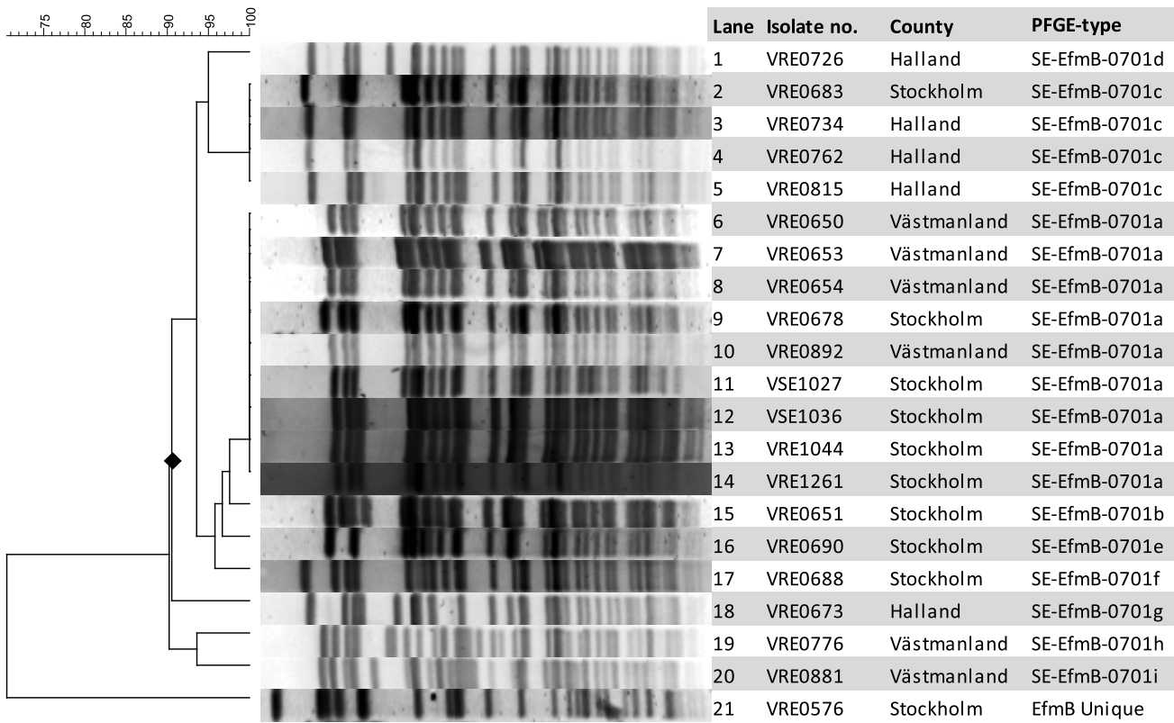
Figure 1. Dendrogram of Smal PFGE of the 21 isolates in collection A. The dendrogram shows that 20 of the isolates are clonal (lane 1–20) and one is divergent (lane 21). The symbol \blacklozenge in the dendrogram indicates a similarity of 90.6%. The PFGE-type nomenclature is based on the following: SE stands for Sweden, EfmB stands for E. faecium with vanB , the number 07 represents year 2007 (the year the index was identified) and the last number is a serial number. The letter at the end describes which PFGE-subtype the isolate belongs to. doi:10.1371/journal.pone.0103274.g001
