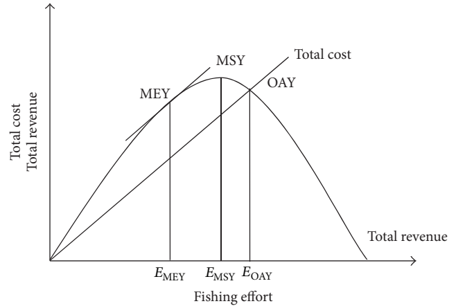
FIGURE 1: The Gordon-Schaefer model.
