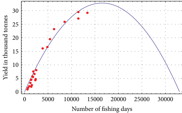
FIGURE 2: Gordon-Schaefer harvest curve for the fishery of 1996 to 2007 based on (14) and catch data from Table 1.
