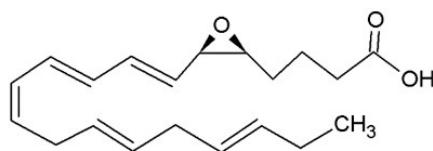
Figure 3. Leukotriene A 5 .
