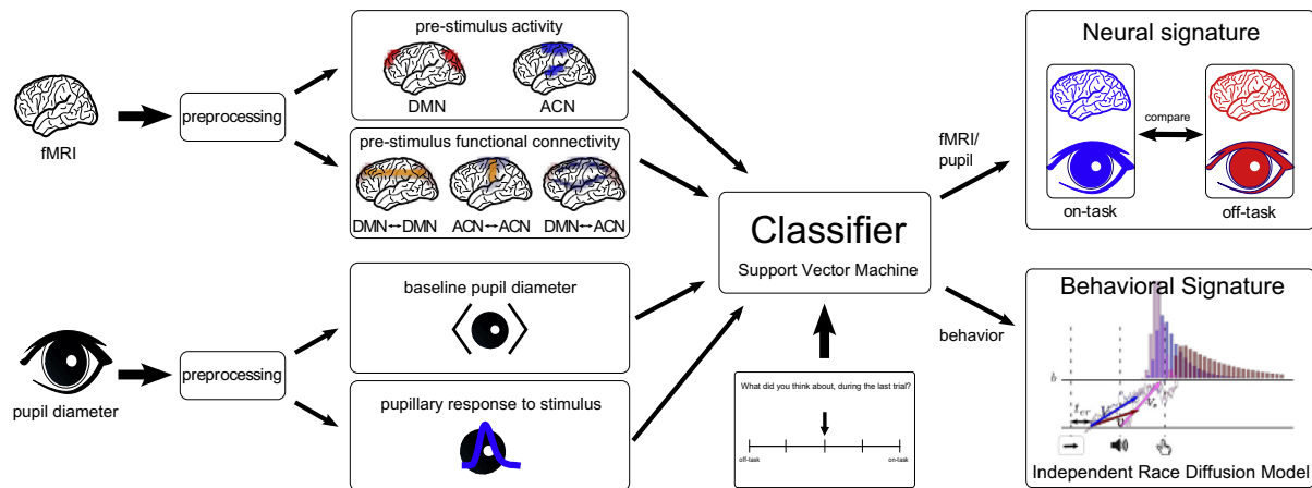
Fig. 2. Summary of Mittner et al.'s (2014) analysis procedure. fMRI and pupil diameter recordings were preprocessed and theoretically derived features were extracted and fed into a machine learning classifier. Self-reported mind wandering scores were used as labels and the classifier was trained to predict them. After training, all trials were classified and the neural and behavioral signature of on-task and off-task behavior was analyzed. Reproduced with permission from Mittner et al. (2014).
