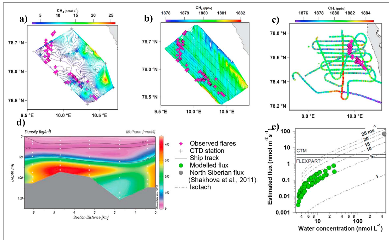
Figure 4. Comparison of CH 4 variations in the ocean and atmosphere west of Svalbard and corresponding CH 4 flux to the atmosphere. (a) Contour plot of near-surface CH 4 concentration (color scale) at ~10 m depth in the water column. CH 4 was measured by oceanographic conductivity-temperature-depth (CTD) stations (crosses) west of Prins Karls Forland (PKF). Observed flares are shown by pink markers. (b) Contour plot of atmospheric CH 4 mixing ratio in parts per billion measured aboard R/V Helmer Hanssen (color scale). Ship track is shown by black line; flares are shown by pink markers. (c) CH 4 measured by the FAAM aircraft; flares are shown by pink markers. (d) CH 4 concentration in the water column along a transect of CTD stations taken on 1 July 2014 showing a clear stratification of water masses with the pycnocline near 50 m water depth. Density is shown as black contours. (The transect location offshore of Prins Karls Forland is shown in Figure S2b). (e) CH 4 flux to the atmosphere at each CTD location as a function of ocean CH 4 concentration according to a diffusive model (green points). Flux previously modeled off Northern Siberia during stormy weather [Shakhova et al. , 2014] is given by the grey point. Dashed lines show the model flux at different isotachs (lines of constant wind speed), assuming constant salinity and temperature (averaged over the sampling period used). Horizontal lines show the maximum possible flux constrained by the atmospheric measurements from the ship, according to FLEXPART and Oslo CTM3 models. FLEXPART and CTM constraints are for the atmospheric sampling period 20 June to 1 August and will vary with weather patterns.
