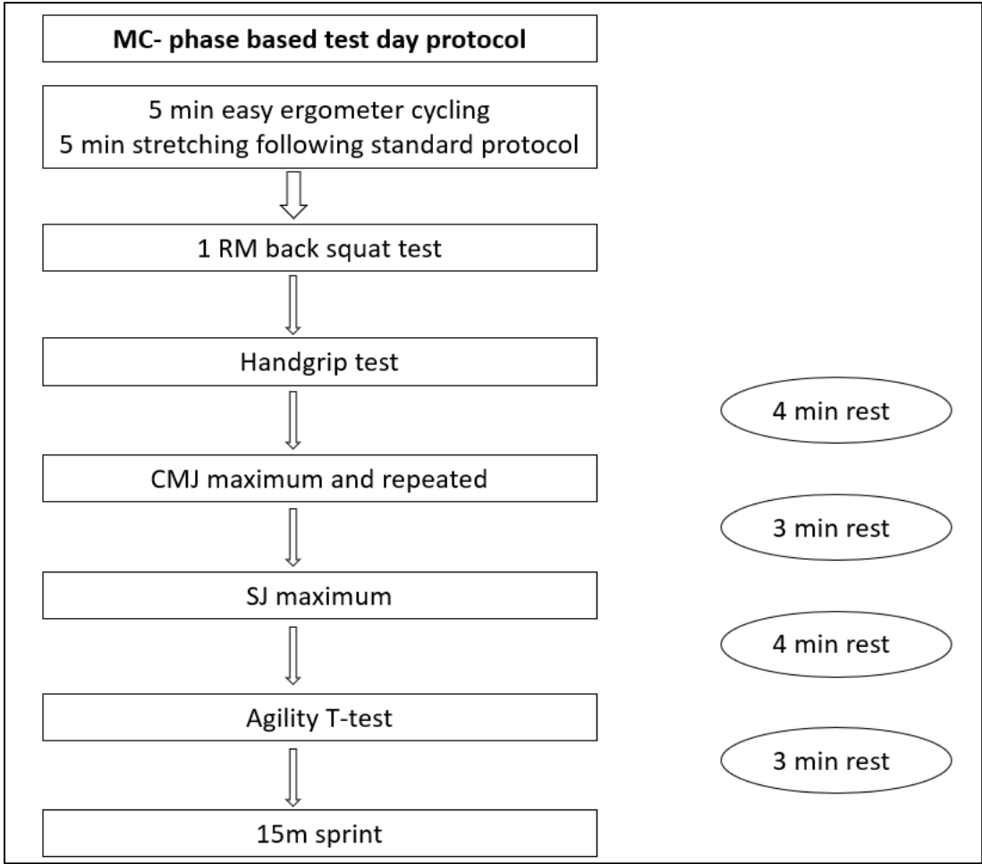
Figure 1. Flow chart display of the protocol followed in the MC-phase based testing for the physical testing in 1 repetition maximum back squat, maximal handgrip strength, countermovement jump (CMJ), squat jump (SJ), agility T-test and 15-m sprint. Abbreviations: MC, menstrual cycle; min, minutes. Abbreviations: MC, menstrual cycle; min, minutes.
