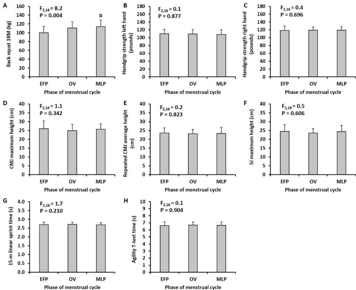
Figure 4. Mean and standard deviation results through phases of the menstrual cycle for A) 1RM back squat, B) handgrip strength left hand, C) handgrip strength right hand, D) maximal CMJ, E) repeated CMJ, F) squat jump, G) 15 m sprint and H) agility. Abbreviations: 1RM, one-repetition maximum; CMJ, counter movement jump; SJ, squat jump; EFP, early follicular phase; OV, ovulation; MLP, mid-luteal phase. α Indicates a significant difference between MLP and EFP in the back squat 1RM.
