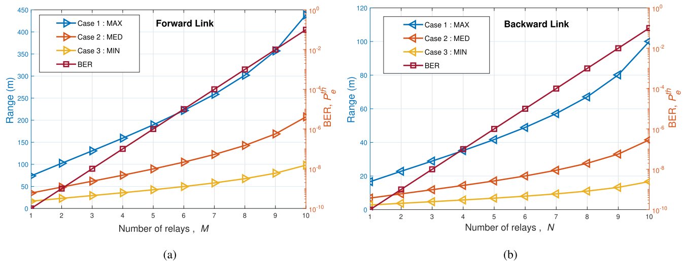
FIGURE 5. Total range for multi-hop system versus a target of BER at different electrical transmit power budgets and different values of bandwidth, for the Forward (a) and Backward (b) links for N, M \in \{1, 2, \dots, 10\} .
